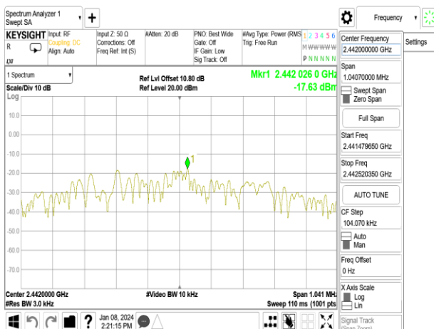
PSD_BLE 1M_MidCH20-2442MHz
