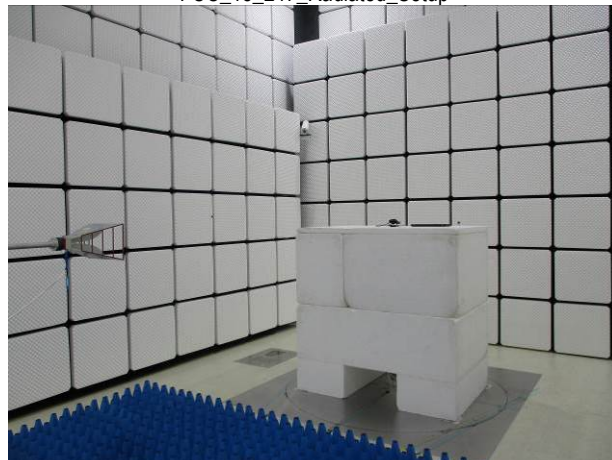
FCC_15_247_Radiated_Setup
