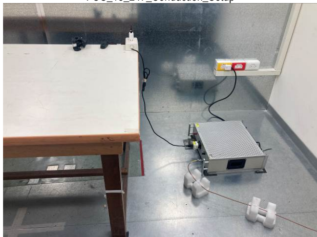
FCC_15_247_Conduction_Setup
