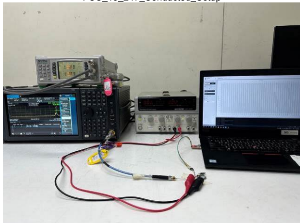
FCC_15_247_Conduction_Setup
