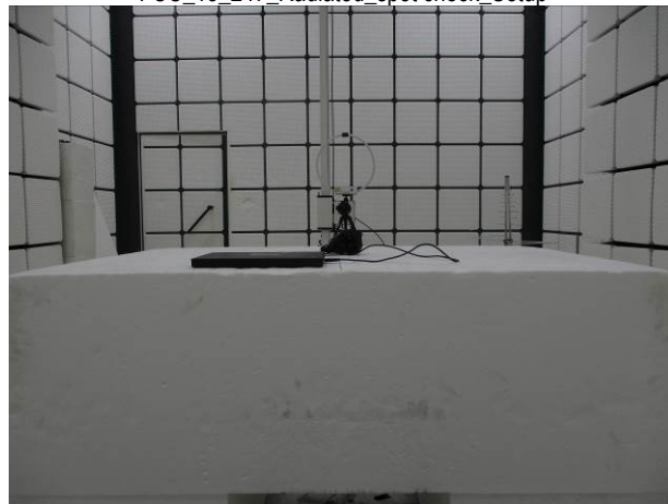
FCC_15_247_Radiated_spot check_Setup
