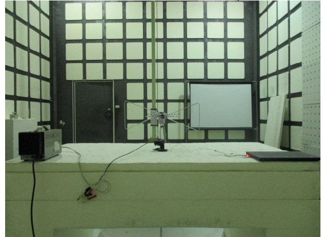
Part_15_247_BLE_Radiated_Setup
