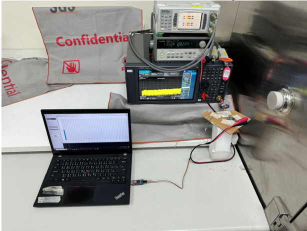
Part_15_247_BLE_Radiated_Setup
