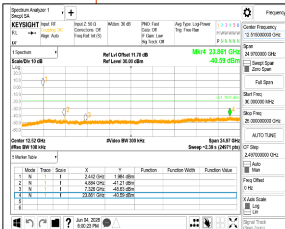
Spurious Emission_BLE 1M_MidCH20-2442MHz
