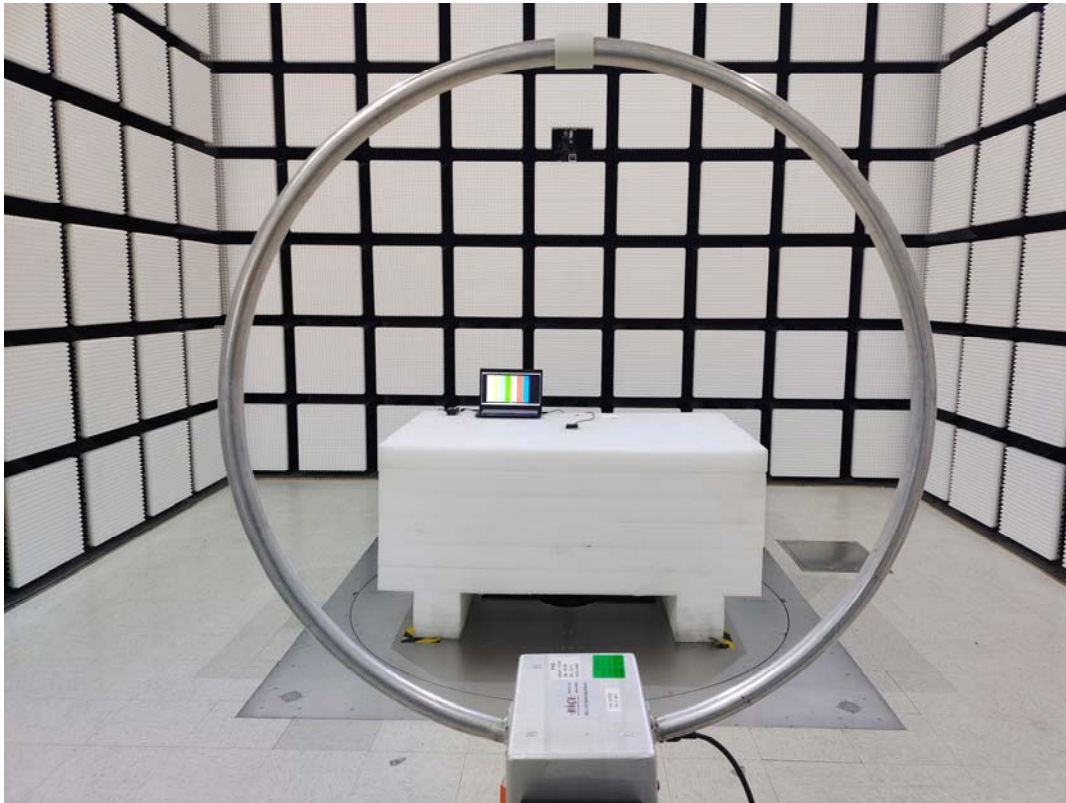
Radiated Emission Below 9 kHz-30 MHz Perpendicular View
