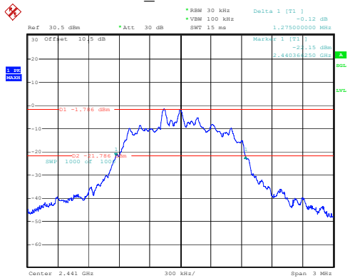
3DH1_Middle 1.275MHz
