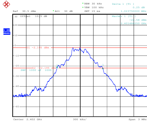
DH1_Low 1.024MHz
