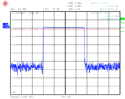
DH1_Hopping 0.389ms
