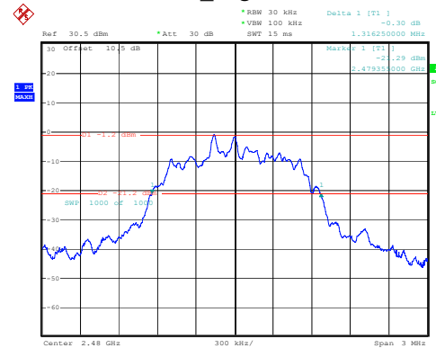
2DH1_High 1.316MHz
