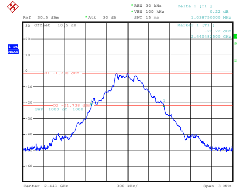
DH1_Middle 1.039MHz
