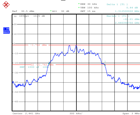
2DH1_Middle 1.313MHz
