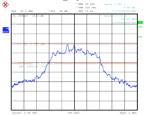
3DH1_High 1.271MHz
