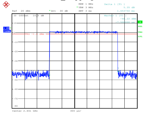
2DH3_Hopping 1.654ms
