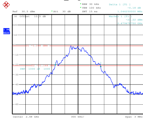
DH1_High 1.046MHz
