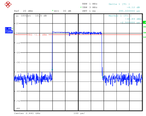
2DH1_Hopping 0.395ms
