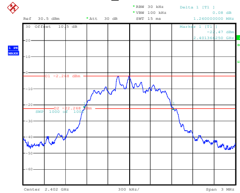
2DH1_Low 1.260MHz
