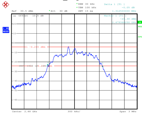
2DH1_High 1.313MHz
