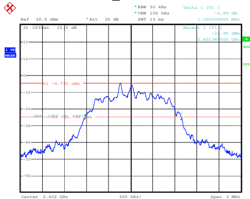
2DH1_Low 1.305MHz
