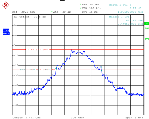
DH1_Middle 1.035MHz
