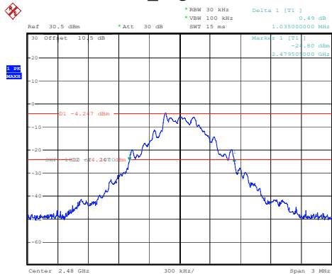
DH1_High 1.035MHz
