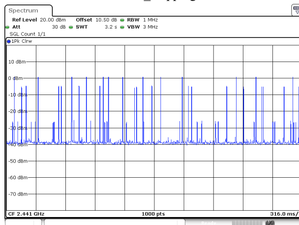
3DH5_Hopping
