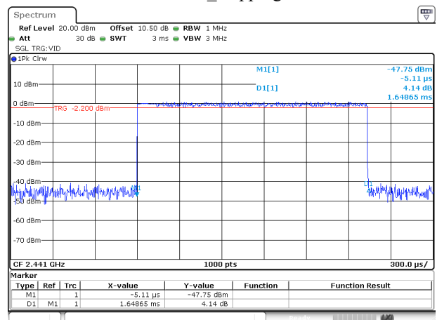
3DH3_Hopping
