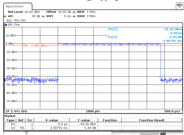
3DH5_Hopping
