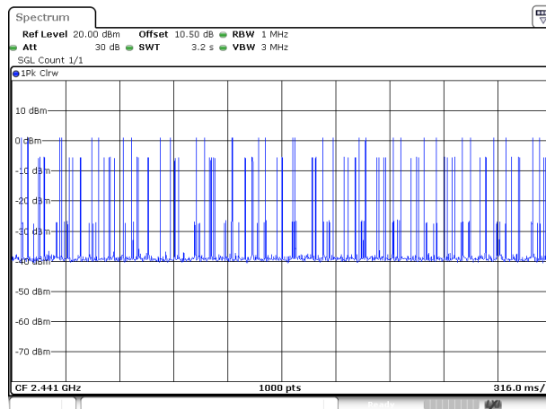
3DH1_Hopping
