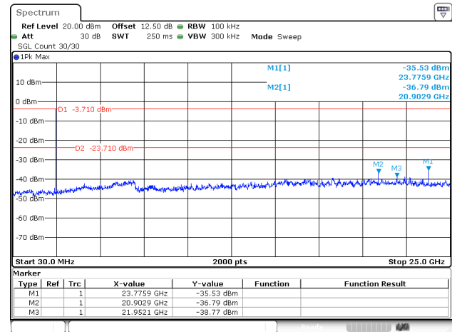
DH1_High
