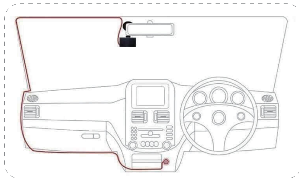
Wiring Method B
