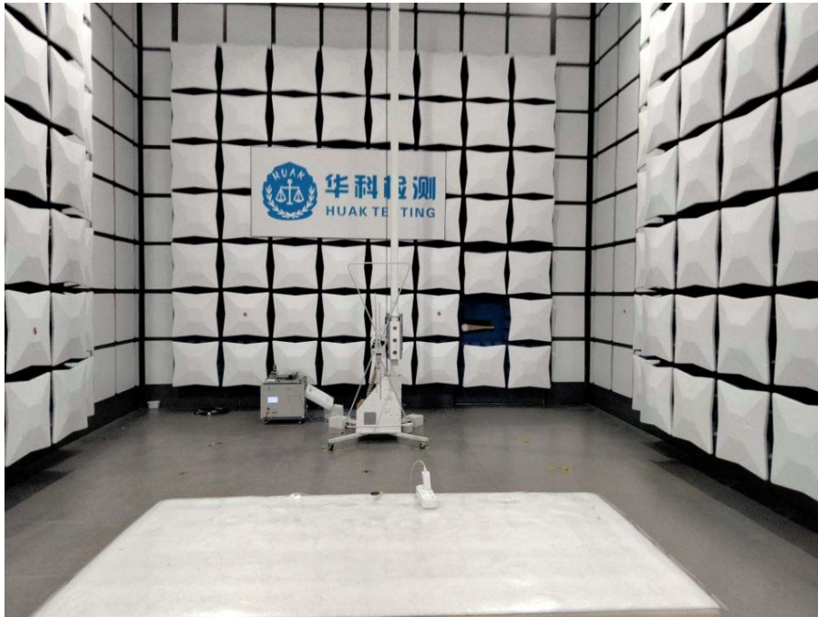
Model: VP-18 Radiated Emissions
