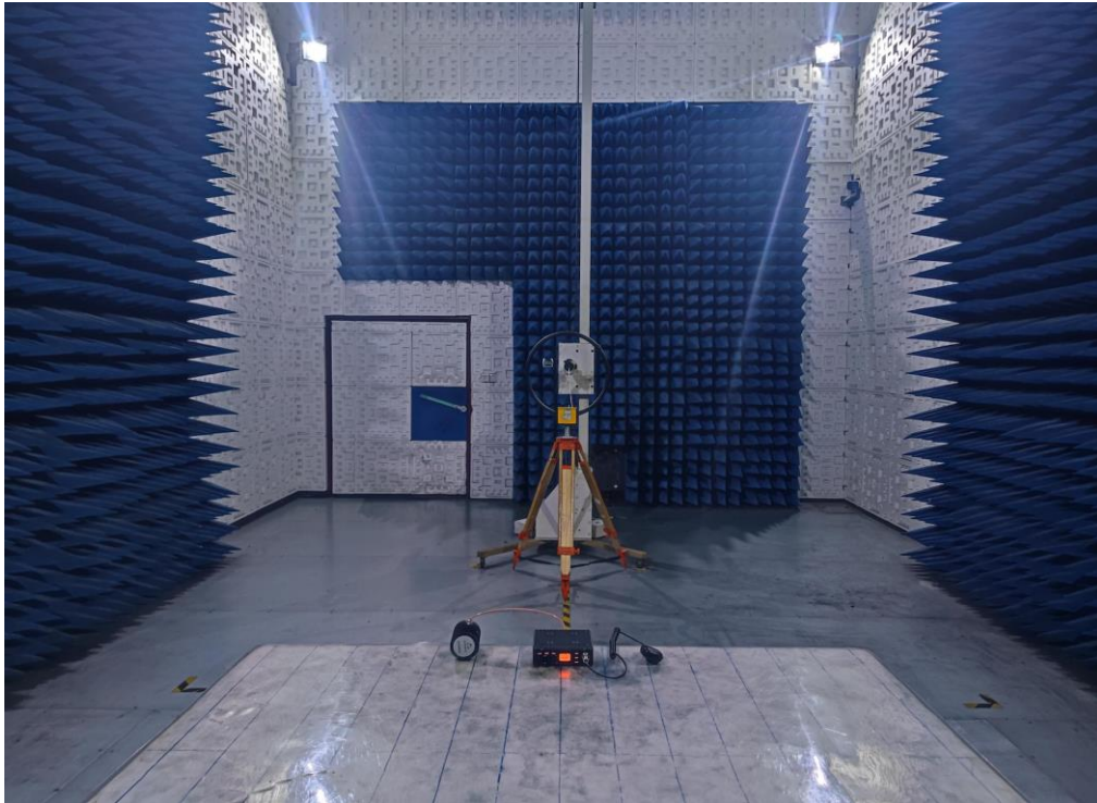
RADIATED EMISSION TEST SETUP BELOW 1GHz
