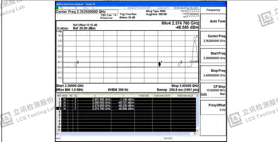
3DH5_BT Ant_Low_2402_Peak
