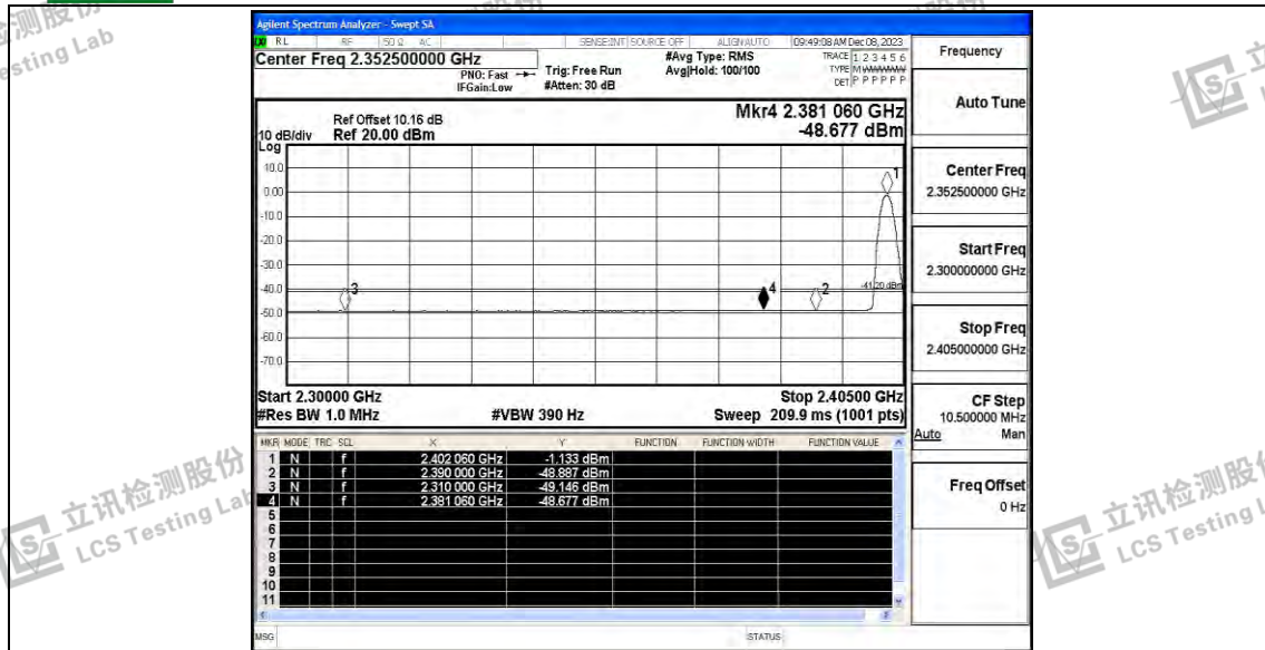
2DH5_BT Ant_Low_2402_Peak
