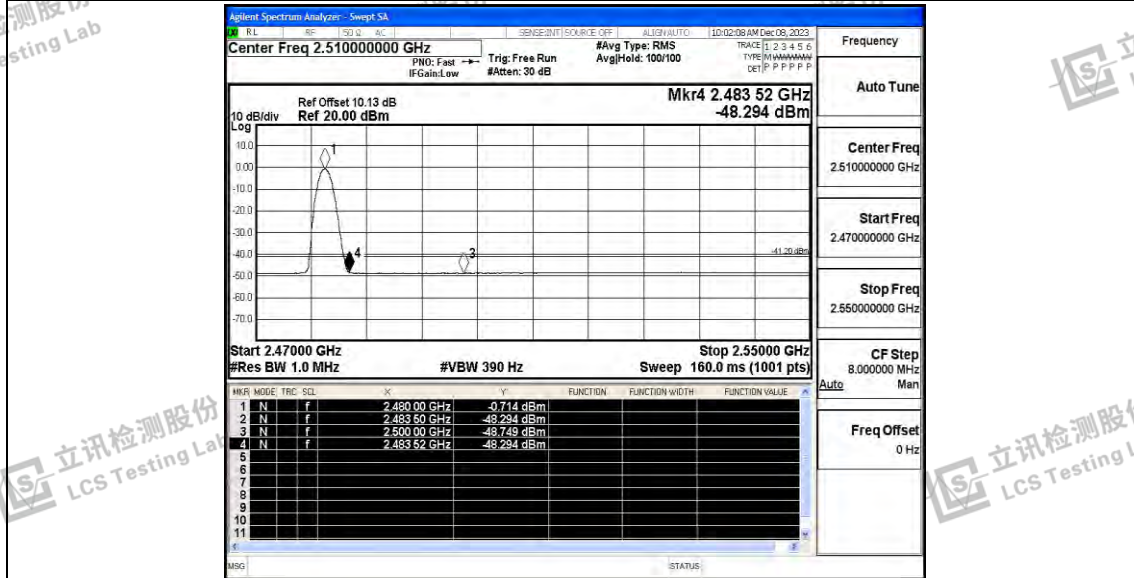
3DH5_BT Ant_High_2480_Peak
