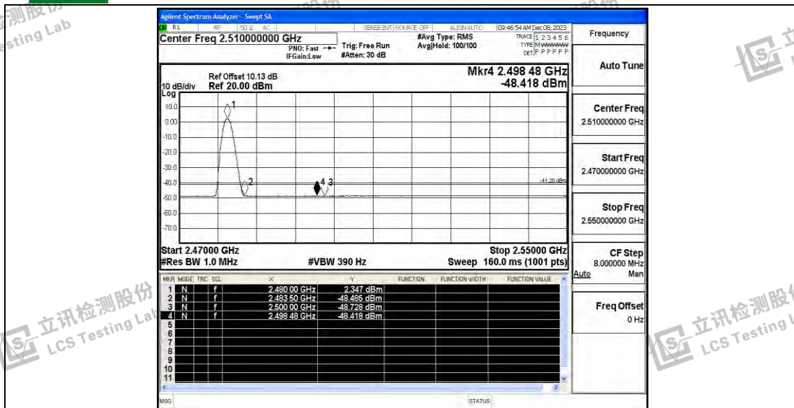
DH5_BT Ant_High_2480_Peak
