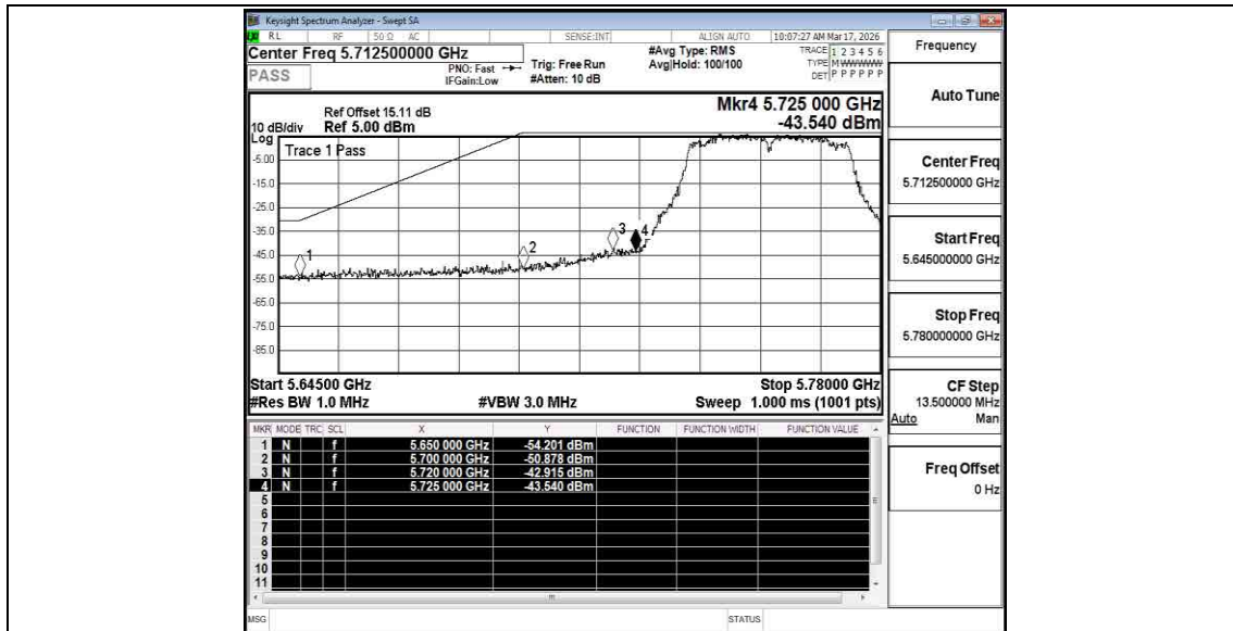
11N40SISO_Ant2_High_5795_Peak
