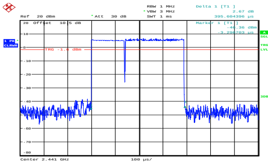
8DPSK_Hopping_3DH1 0.396ms
