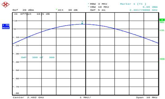
8DPSK_Low 5.66dBm
