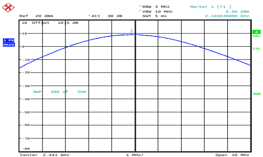
GFSK_Middle 8.86dBm
