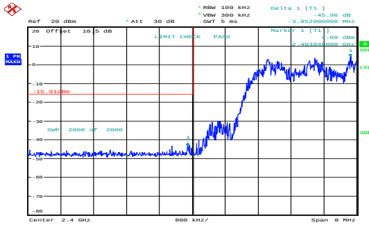
8DPSK_Hopping_Lower 45.96dB
