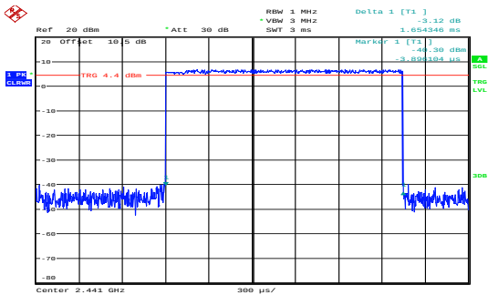
8DPSK_Hopping_3DH3 1.654ms
