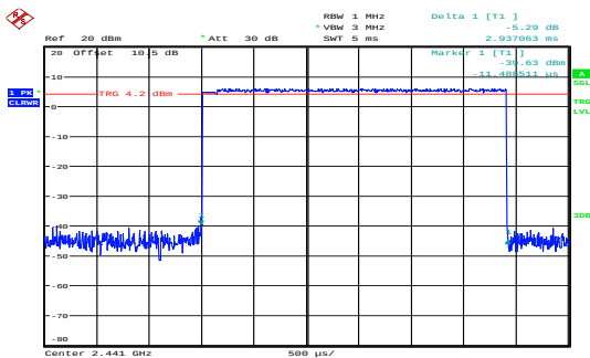
8DPSK_Hopping_3DH5 2.937ms
