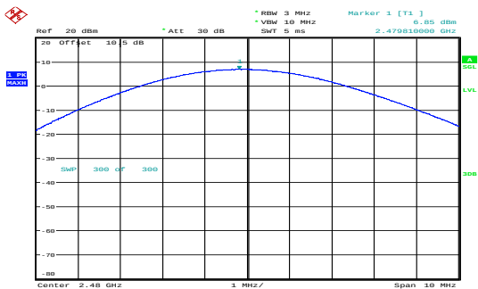
8DPSK_High 6.85dBm
