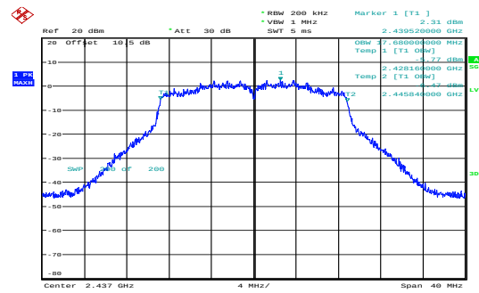
n20_2437MHz_Chain 0 17.680MHz
