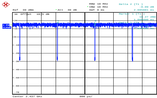
g_2437MHz_Chain 0 2.035ms,2.086ms
