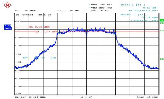
g_2412MHz_Chain 0 15.225MHz
