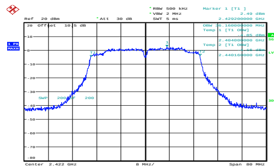
n40_2422MHz_Chain 0 36.160MHz
