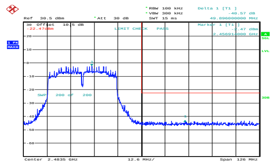
n40_2452MHz_Chain 1 40.57dB
