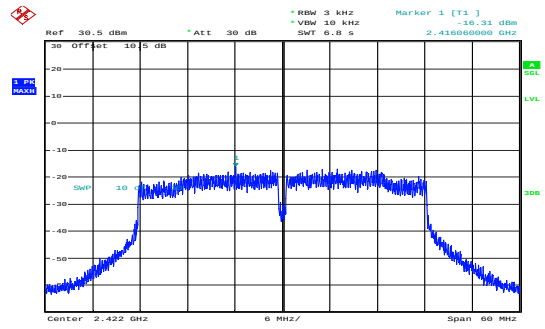
n40_2422MHz_Chain 1 -16.31dBm/3kHz
