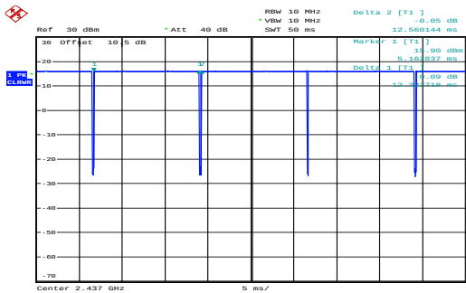
b_2437MHz_Chain 0 12.324ms,12.560ms
