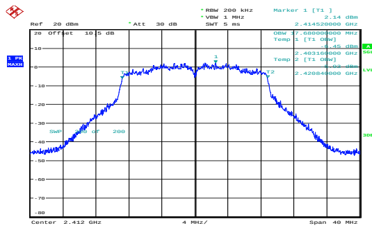
n20_2412MHz_Chain 0 17.680MHz
