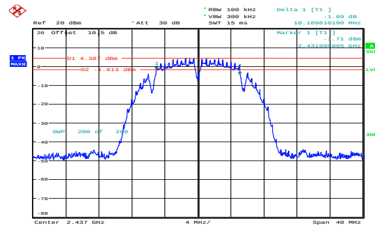
b_2437MHz_Chain 0 10.190MHz
