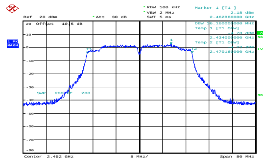
n40_2452MHz_Chain 0 36.160MHz
