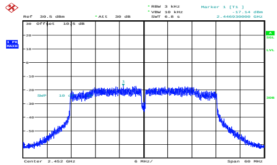
n40_2452MHz_Chain 1 -17.14dBm/3kHz
