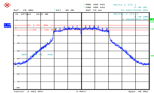
g_2462MHz_Chain 0 15.225MHz
