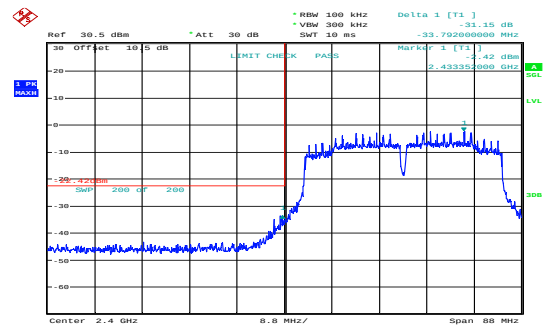
n40_2422MHz_Chain 1 31.15dB
