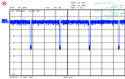
n20_2437MHz_Chain 0 0.967ms,1.020ms
