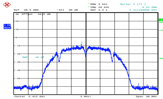
b_2412MHz_Chain 1 -9.25dBm/3kHz
