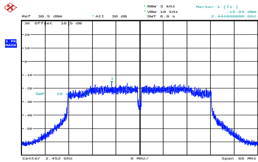
n40_2452MHz_Chain 0 -15.93dBm/3kHz
