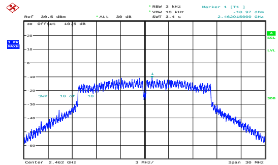
g_2462MHz_Chain 1 -10.97dBm/3kHz
