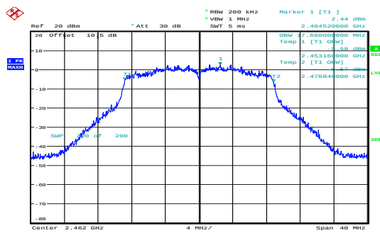
n20_2462MHz_Chain 0 17.680MHz
