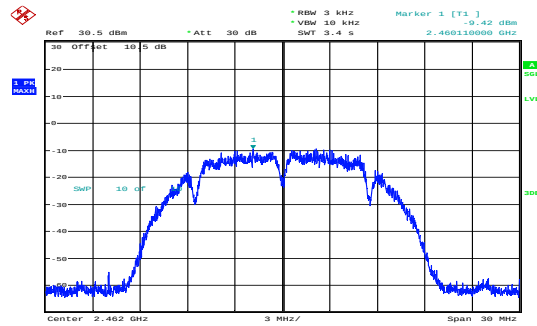
b_2462MHz_Chain 1 -9.42dBm/3kHz
