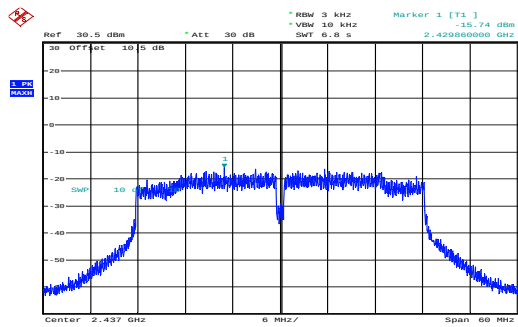
n40_2437MHz_Chain 0 -15.74dBm/3kHz
