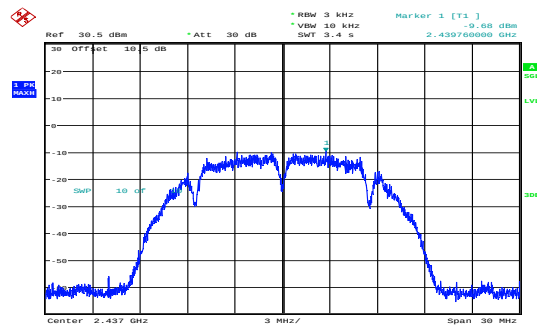
b_2437MHz_Chain 1 -9.68dBm/3kHz
