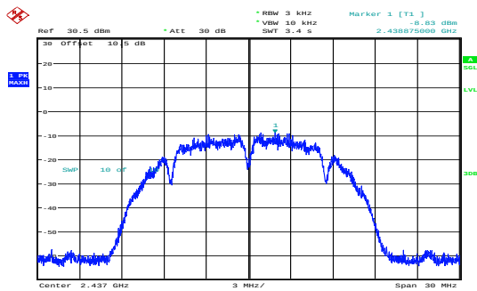
b_2437MHz_Chain 0 -8.83dBm/3kHz
