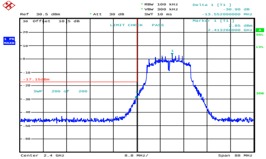
g_2412MHz_Chain 0 30.90dB
