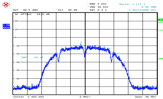
b_2462MHz_Chain 0 -9.05dBm/3kHz
