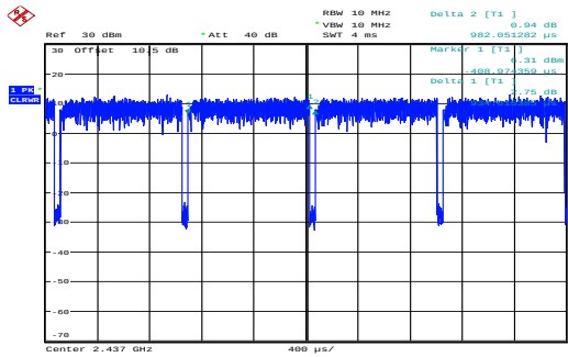
n40_2437MHz_Chain 0 0.935ms,0.982ms
