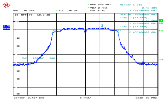
n40_2437MHz_Chain 0 36.160MHz
