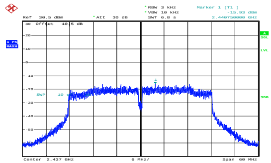
n40_2437MHz_Chain 1 -15.93dBm/3kHz
