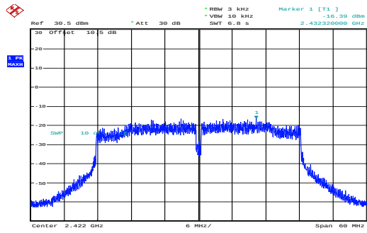
n40_2422MHz_Chain 0 -16.39dBm/3kHz
