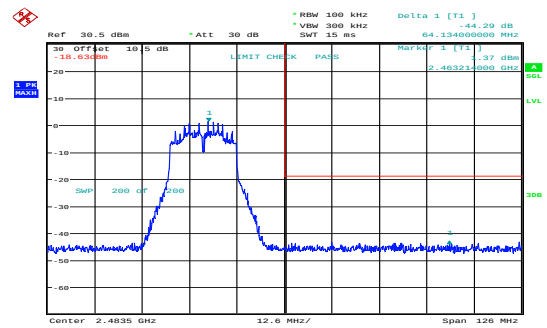
n20_2462MHz_Chain 1 44.29dB
