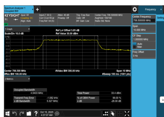
Band17-5MHz-QPSK-23755-25RB#0-PASS
