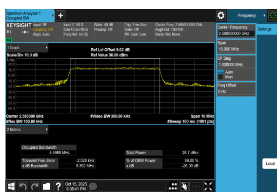
Band38-5MHz-16QAM-38000-25RB#0-PASS
