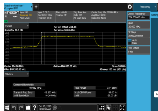
Band12-10MHz-QPSK-23060-50RB#0-PASS
