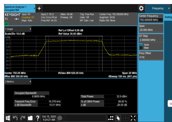
Band13-10MHz-QPSK-23230-50RB#0-PASS
