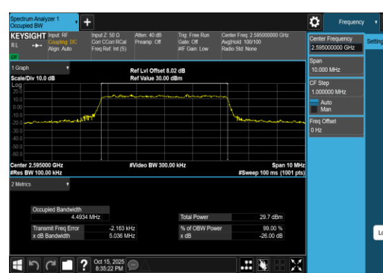
Band38-5MHz-QPSK-38000-25RB#0-PASS
