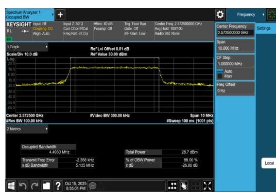
Band38-5MHz-16QAM-37775-25RB#0-PASS
