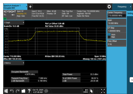
Band17-5MHz-QPSK-23790-25RB#0-PASS
