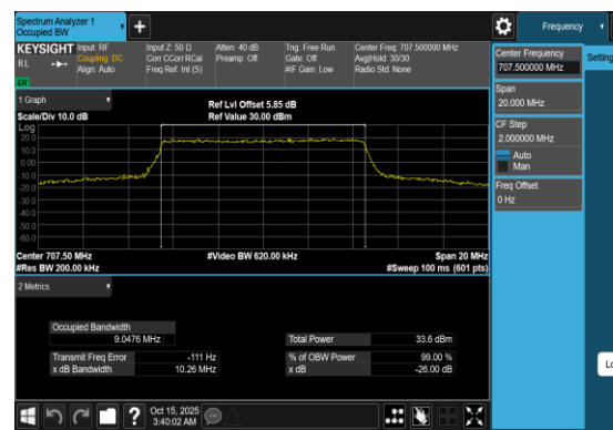
Band12-10MHz-QPSK-23095-50RB#0-PASS
