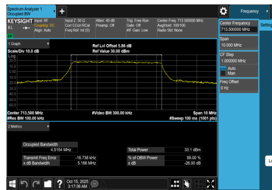
Band12-5MHz-QPSK-23155-25RB#0-PASS
