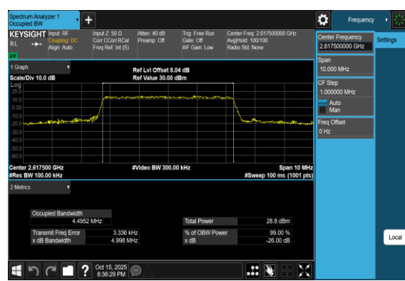
Band38-5MHz-16QAM-38225-25RB#0-PASS
