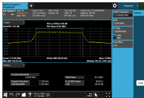
Band12-5MHz-16QAM-23155-25RB#0-PASS
