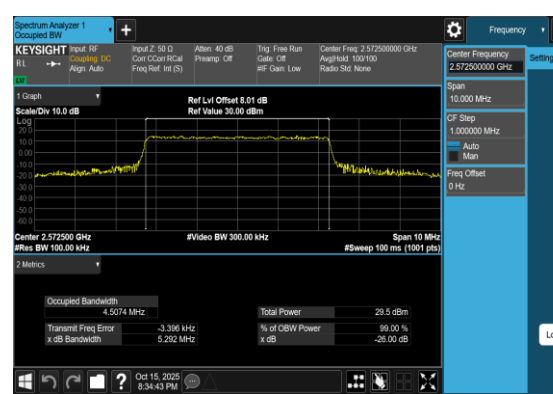
Band38-5MHz-QPSK-37775-25RB#0-PASS
