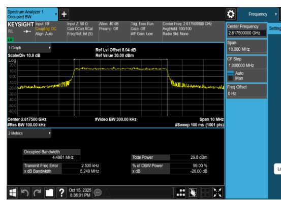
Band38-5MHz-QPSK-38225-25RB#0-PASS
