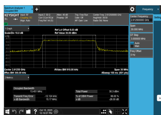
Band38-15MHz-QPSK-38175-75RB#0-PASS
