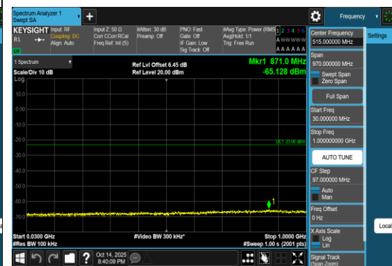
Band2_1.4MHz_16QAM_19193_1RB#0_30~1000_30~1000
