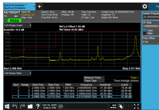
Band41_15MHz_QPSK_39725_1RB#74
