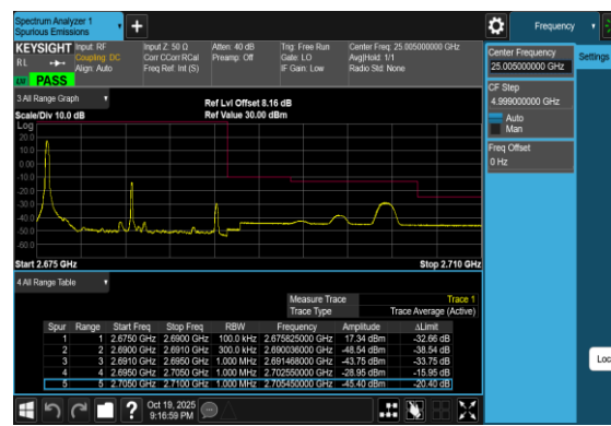
Band41_15MHz_16QAM_41515_1RB#0
