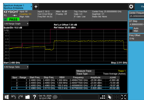
Band41_15MHz_16QAM_39725_75RB#0
