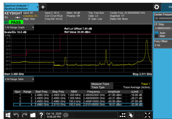
Band41_15MHz_16QAM_39725_1RB#74
