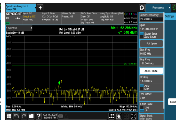
Band2_1.4MHz_16QAM_19193_1RB#0_0.009~0.15_0.009~0.15
