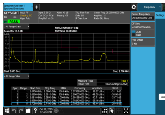
Band41_15MHz_QPSK_41515_1RB#0
