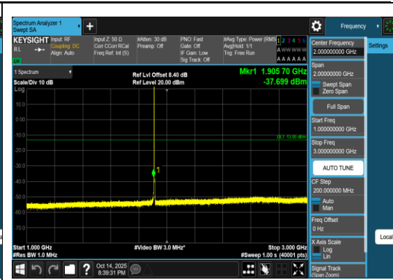
Band2_1.4MHz_QPSK_19193_1RB#0_1000~300_0_1000~3000
