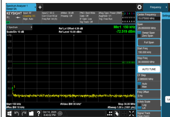
Band2_1.4MHz_16QAM_19193_1RB#0_0.15~30_0.15~30
