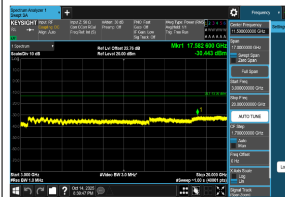
Band2_1.4MHz_QPSK_19193_1RB#0_3000~200_00_3000~20000
