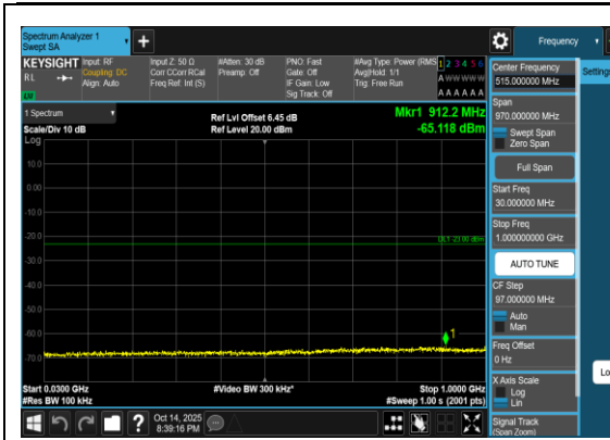
Band2_1.4MHz_QPSK_19193_1RB#0_30~1000_30~1000
