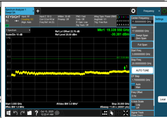
Band4_15MHz_16QAM_20325_1RB#0_3000~20000 00_3000~20000
