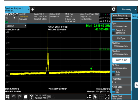
Band4_15MHz_16QAM_20325_1RB#0_1000~3000 00_1000~3000
