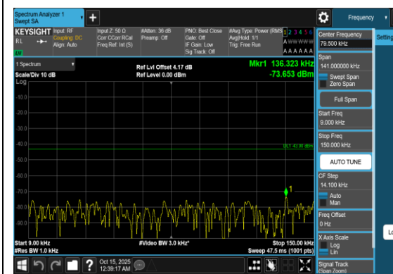
Band4_20MHz_QPSK_20050_1RB#0_0.009~0.1 5_0.009~0.15
