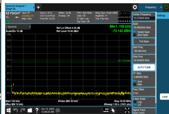
Band4_20MHz_QPSK_20050_1RB#0_0.15~30_0.15~30
