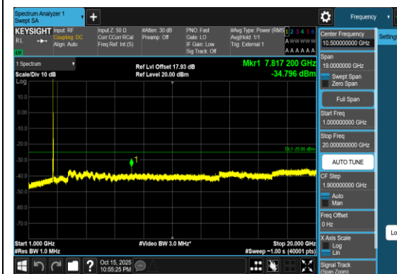
Band38_15MHz_16QAM_38175_1RB#0_1000~20000_1000_1000~20000
