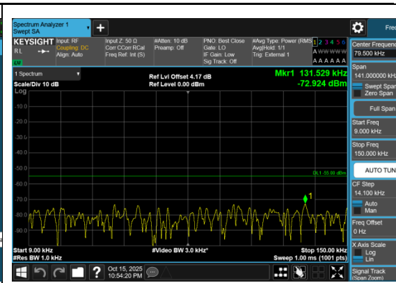
Band38_15MHz_16QAM_38175_1RB#0_0.009~0.15_0.009~0.15
