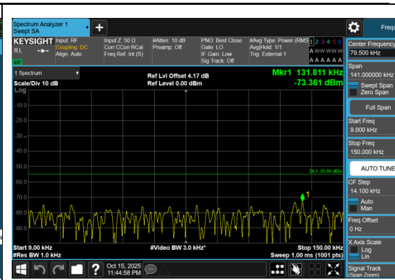
Band38_20MHz_16QAM_38150_1RB#0_0.009~0.15_0.009~0.15
