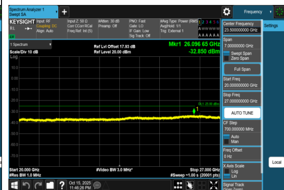
Band38_20MHz_16QAM_38150_1RB#0_2000~27000_7000_20000~27000
