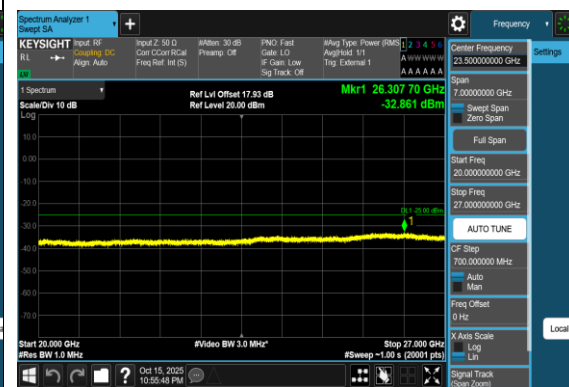
Band38_15MHz_16QAM_38175_1RB#0_20000~27000_7000_20000~27000
