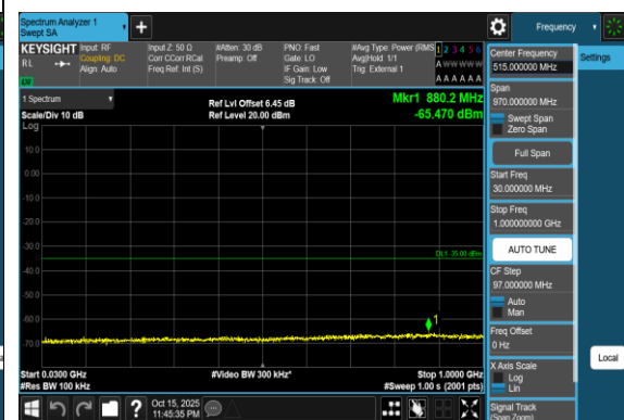
Band38_20MHz_16QAM_38150_1RB#0_30~1000_30~1000
