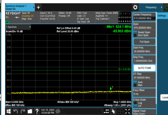
Band38_15MHz_16QAM_38175_1RB#0_30~1000_30~1000
