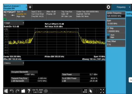
Band5-5MHz-QPSK-20425-25RB#0-PASS
