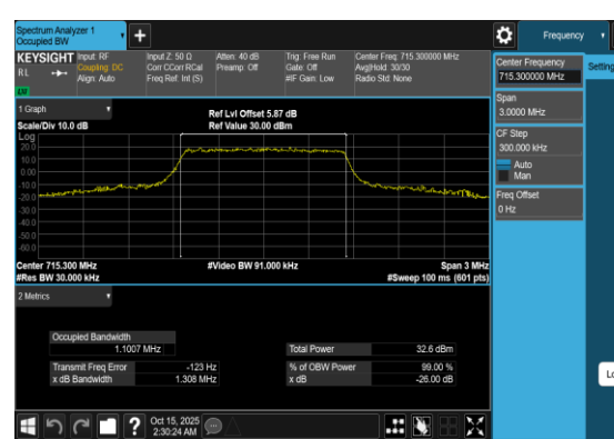
Band12-1.4MHz-QPSK-23173-6RB#0-PASS
