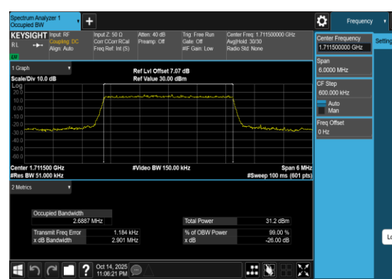
Band4-3MHz-QPSK-19965-15RB#0-PASS
