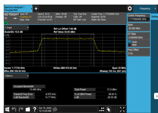
Band4-15MHz-QPSK-20025-75RB#0-PASS
