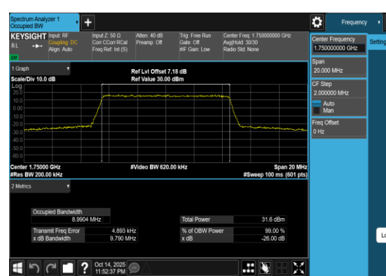
Band4-10MHz-QPSK-20350-50RB#0-PASS
