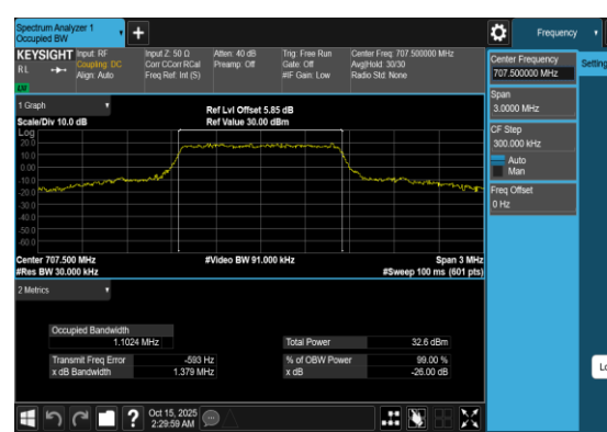
Band12-1.4MHz-QPSK-23095-6RB#0-PASS
