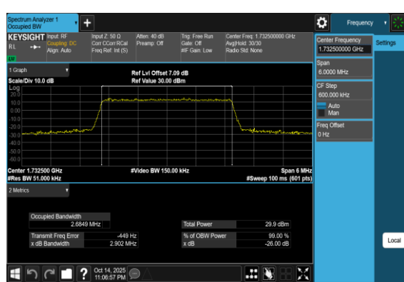
Band4-3MHz-16QAM-20175-15RB#0-PASS
