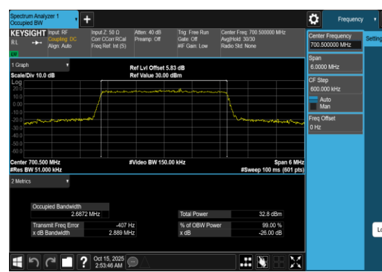
Band12-3MHz-QPSK-23025-15RB#0-PASS
