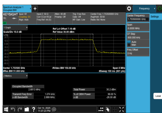
Band4-3MHz-16QAM-20385-15RB#0-PASS
