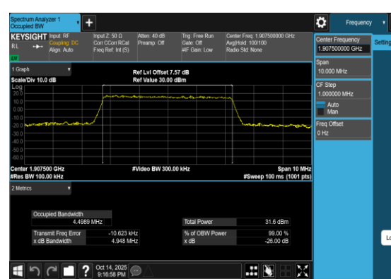
Band2-5MHz-QPSK-19175-25RB#0-PASS
