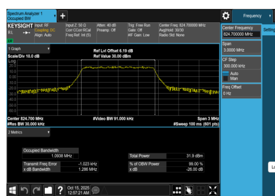
Band5-1.4MHz-QPSK-20407-6RB#0-PASS
