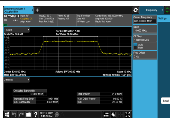
Band5-5MHz-16QAM-20525-25RB#0-PASS
