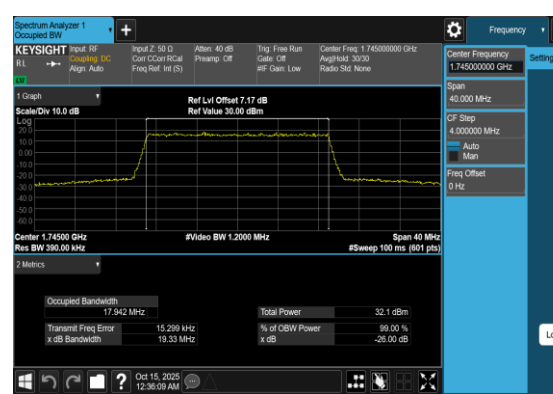
Band4-20MHz-QPSK-20300-100RB#0-PASS
