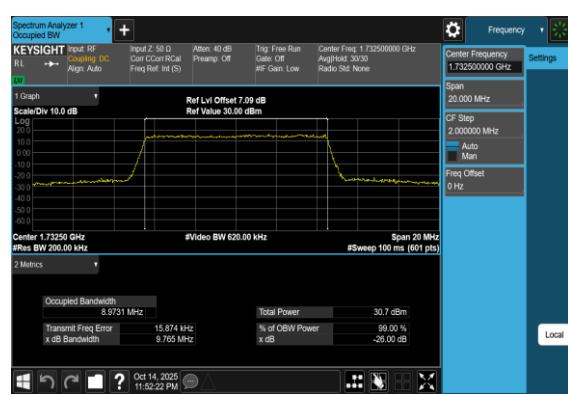
Band4-10MHz-16QAM-20175-50RB#0-PASS
