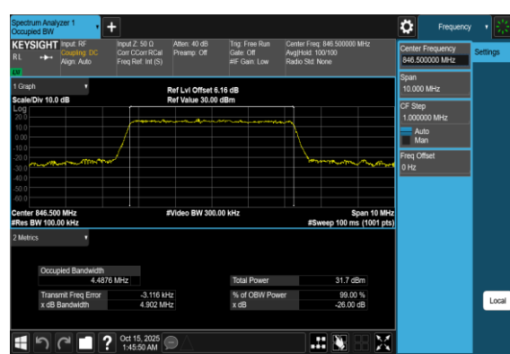
Band5-5MHz-16QAM-20625-25RB#0-PASS
