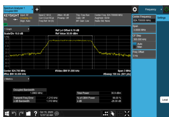
Band5-1.4MHz-16QAM-20407-6RB#0-PASS
