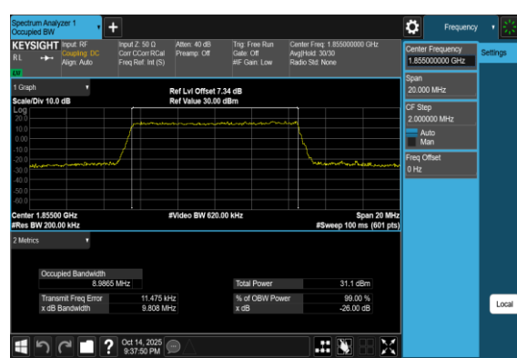
Band2-10MHz-16QAM-18650-50RB#0-PASS
