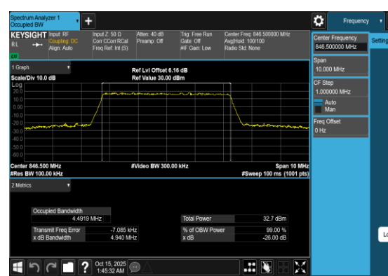
Band5-5MHz-QPSK-20625-25RB#0-PASS
