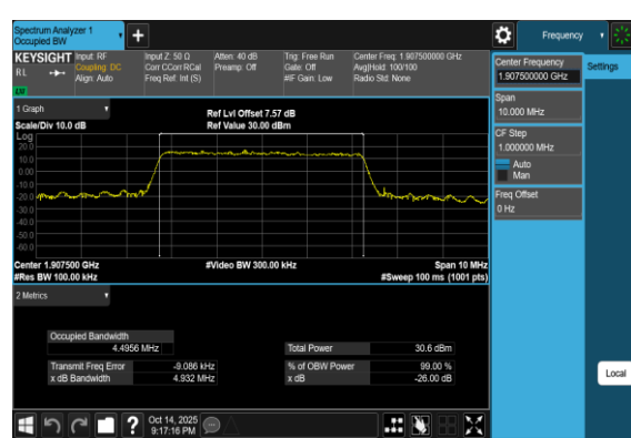
Band2-5MHz-16QAM-19175-25RB#0-PASS
