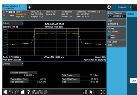
Band4-3MHz-16QAM-19965-15RB#0-PASS
