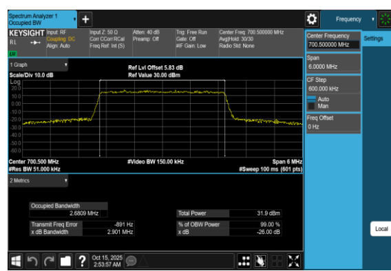
Band12-3MHz-16QAM-23025-15RB#0-PASS
