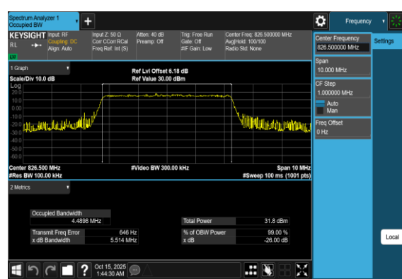
Band5-5MHz-16QAM-20425-25RB#0-PASS
