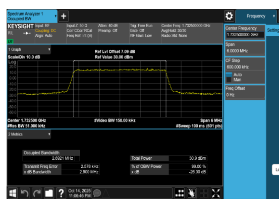
Band4-3MHz-QPSK-20175-15RB#0-PASS
