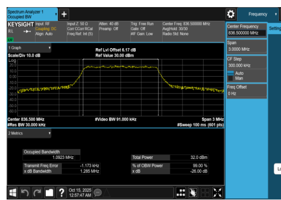
Band5-1.4MHz-QPSK-20525-6RB#0-PASS
