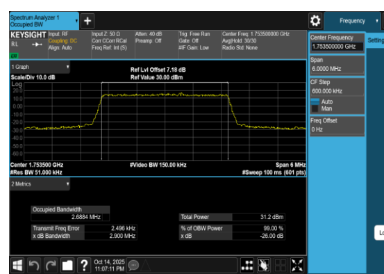
Band4-3MHz-QPSK-20385-15RB#0-PASS
