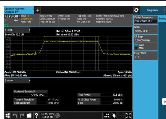
Band5-5MHz-QPSK-20525-25RB#0-PASS
