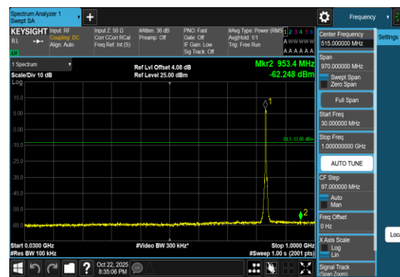
Band5-4182-30~1000MHz-PASS
