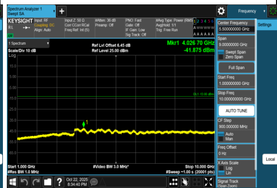
Band5-4132-1000~10000MHz-PASS
