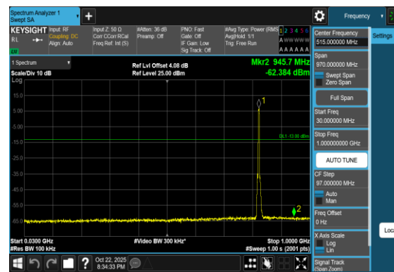
Band5-4132-30~1000MHz-PASS
