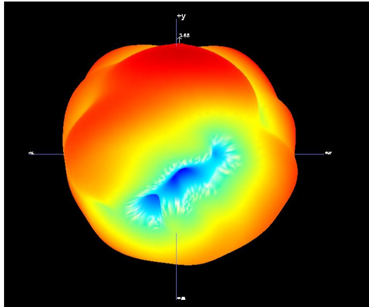
B1.1 3D Pattern for 2400MHz
