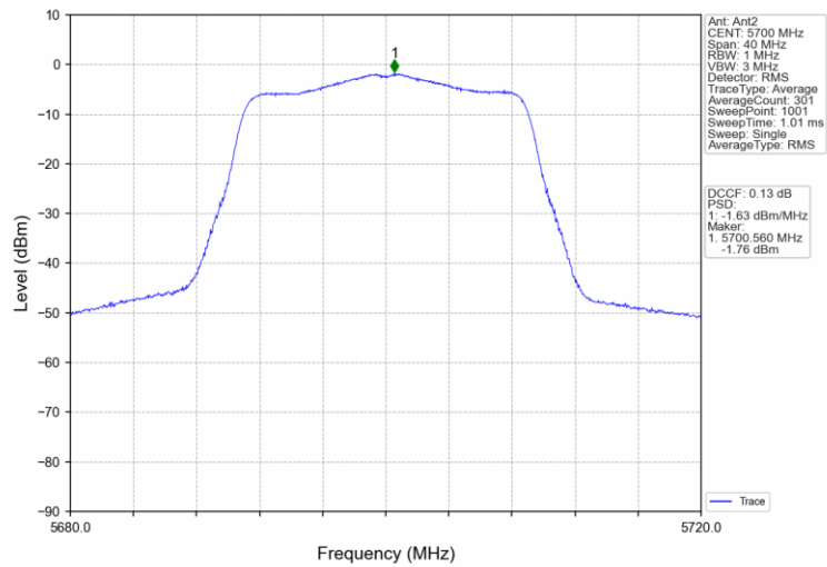
802.11n(HT20)_HCH_5700MHz_MIMO_NTNV
