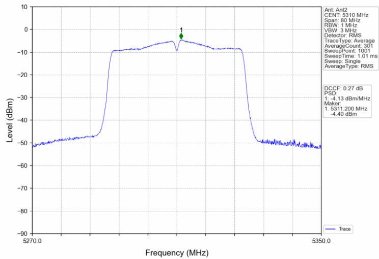
802.11n(HT40)_HCH_5310MHz_MIMO_NTNV
