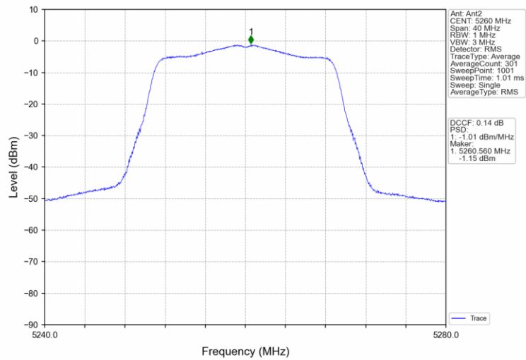
802.11n(HT20)_LCH_5260MHz_MIMO_NTNV
