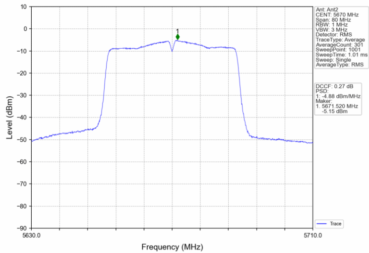
802.11n(HT40)_HCH_5670MHz_MIMO_NTNV
