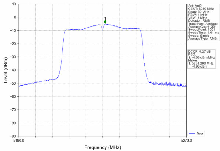
802.11n(HT40)_HCH_5230MHz_MIMO_NTNV
