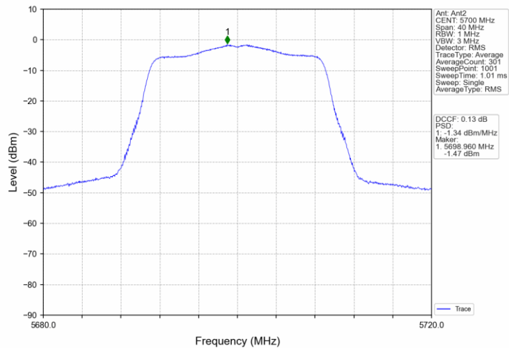
802.11ac(VHT20)_HCH_5700MHz_MIMO_NTNV
