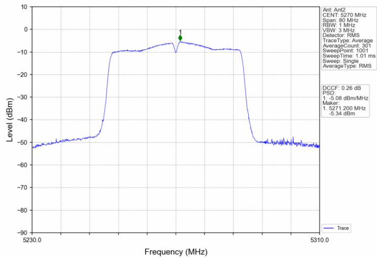
802.11ac(VHT40)_LCH_5270MHz_MIMO_NTNV
