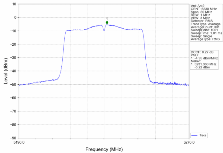
802.11ac(VHT40)_HCH_5230MHz_MIMO_NTNV
