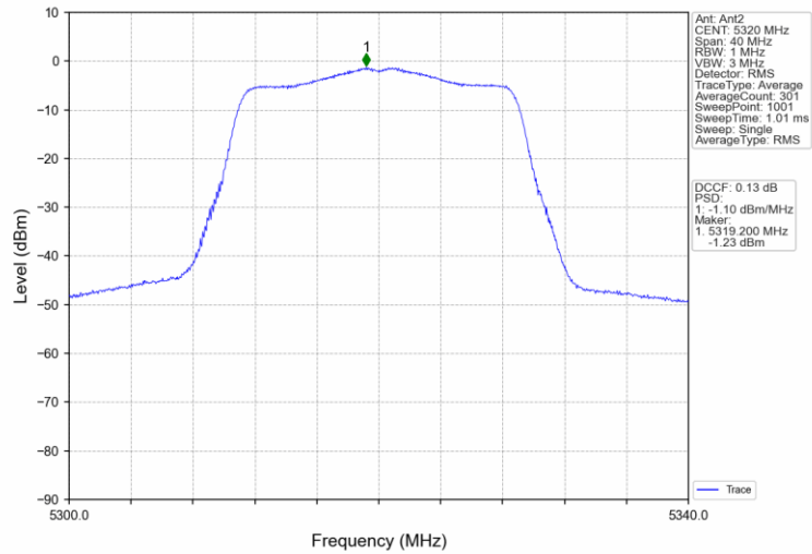
802.11ac(VHT20)_HCH_5320MHz_MIMO_NTNV
