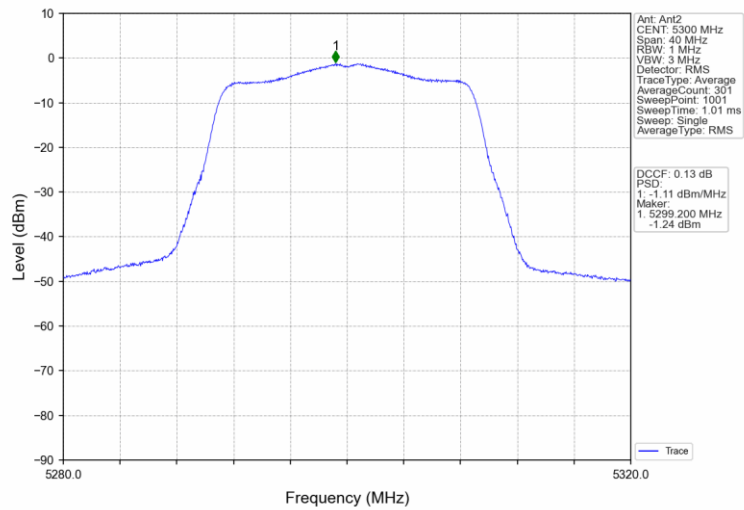
802.11ac(VHT20)_MCH_5300MHz_MIMO_NTNV
