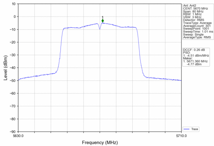
802.11ac(VHT40)_HCH_5670MHz_MIMO_NTNV
