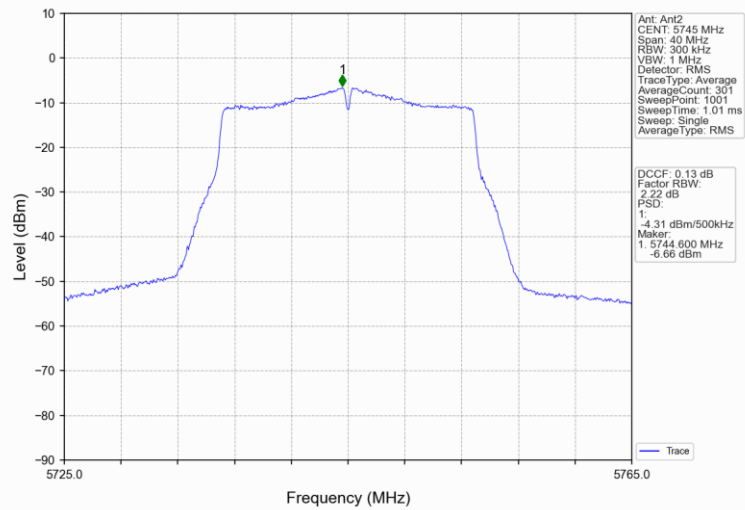
802.11n(HT20)_LCH_5745MHz_MIMO_NTNV
