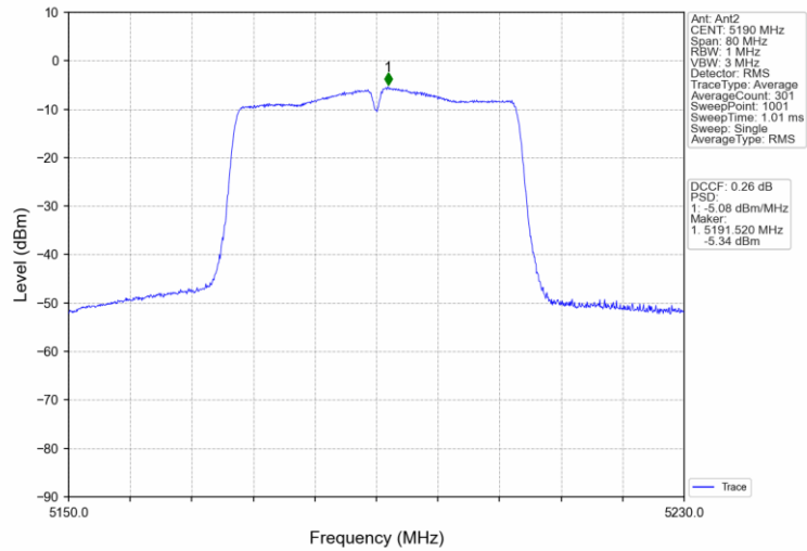
802.11ac(VHT40)_LCH_5190MHz_MIMO_NTNV
