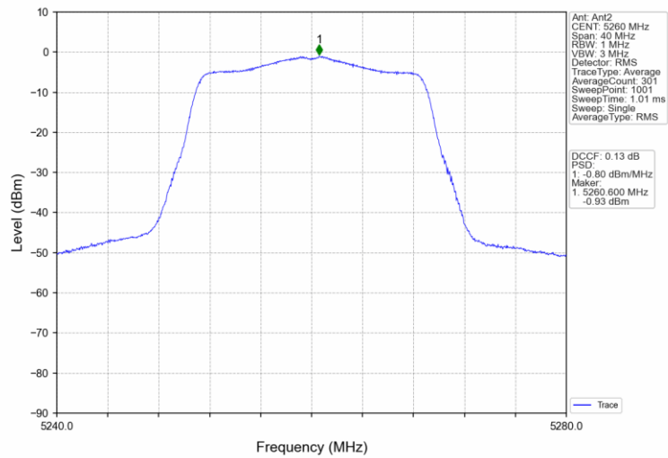
802.11ac(VHT20)_LCH_5260MHz_MIMO_NTNV
