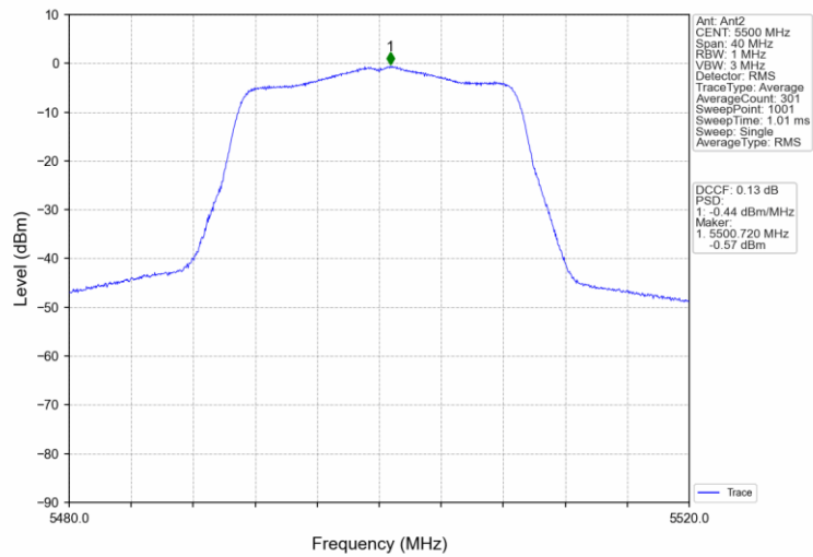
802.11ac(VHT20)_LCH_5500MHz_MIMO_NTNV
