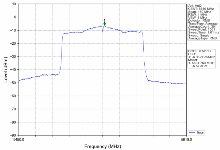
802.11ac(VHT80)_LCH_5530MHz_MIMO_NTNV
