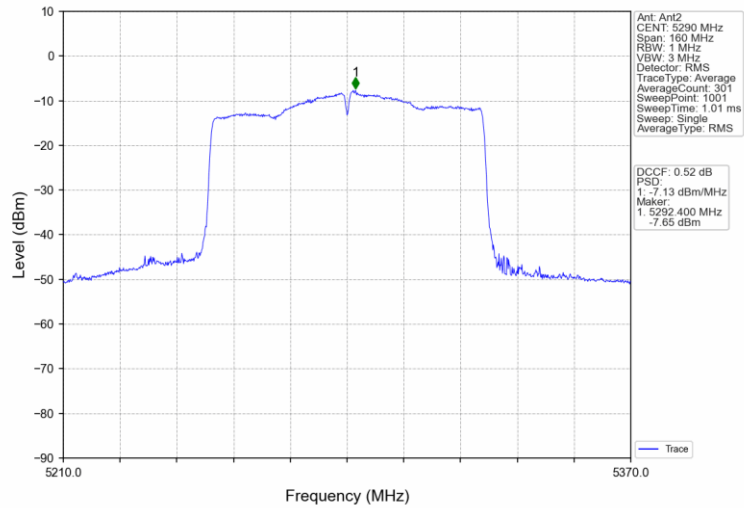
802.11ac(VHT80)_MCH_5290MHz_MIMO_NTNV
