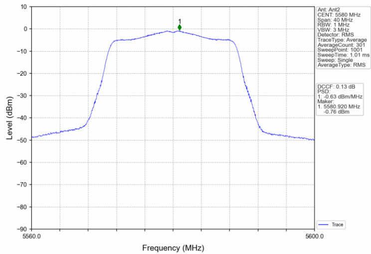
802.11ac(VHT20)_MCH_5580MHz_MIMO_NTNV
