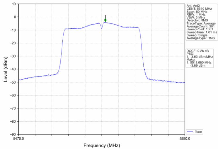
802.11ac(VHT40)_LCH_5510MHz_MIMO_NTNV
