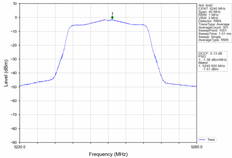
802.11ac(VHT20)_HCH_5240MHz_MIMO_NTNV
