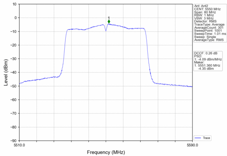
802.11ac(VHT40)_MCH_5550MHz_MIMO_NTNV
