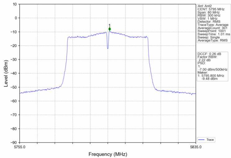
802.11ac(VHT40)_HCH_5795MHz_MIMO_NTNV
