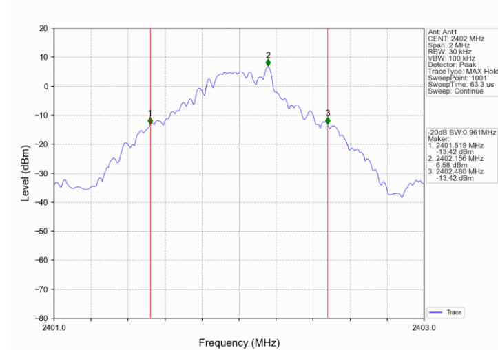
GFSK_DH5_LCH_2402MHz_Ant1_NTNV
