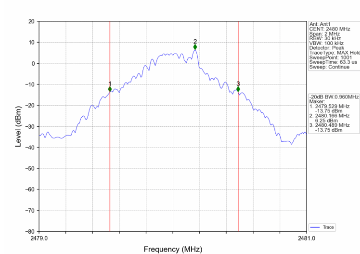
GFSK_DH5_HCH_2480MHz_Ant1_NTNV
