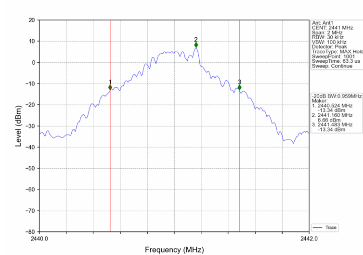
GFSK_DH5_MCH_2441MHz_Ant1_NTNV
