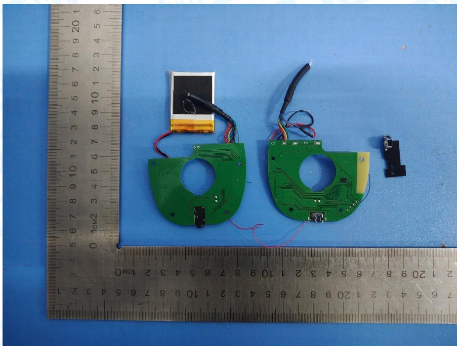
Photo 18 Appearance of PCB& Battery
