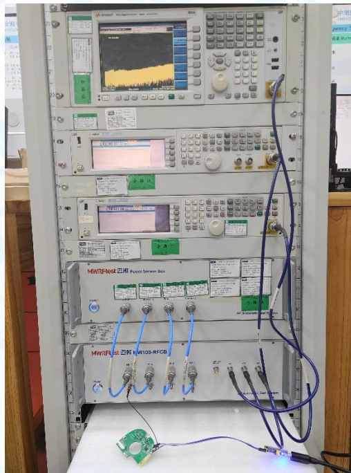
Photo of Setup for RF Conducted Measurements
