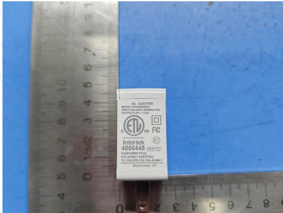
Photo 8 2#Adapter Appearance
