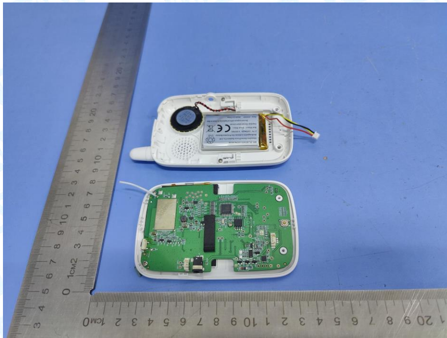
Photo 11 Internal of EUT (Differential prototype)
