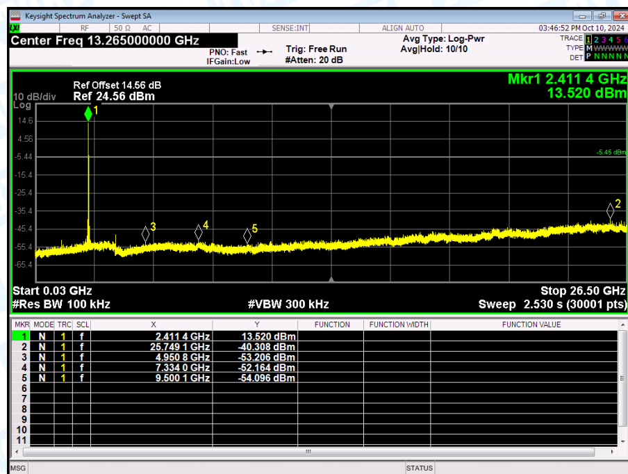
Tx. Spurious NVNT user 2412MHz Ant1 Emission
