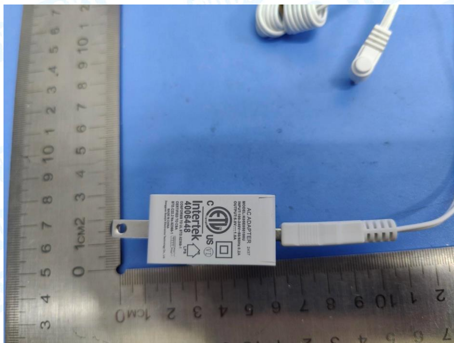
Photo 10 Adapter Appearance 3#
