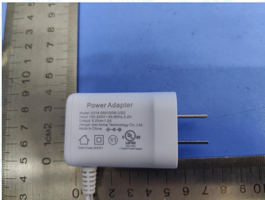
Photo 12 Adapter Appearance 5#
