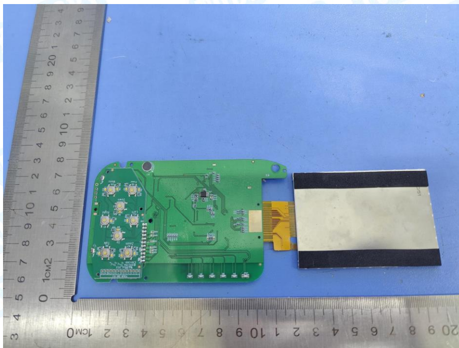
Photo 18 Appearance of PCB Differential prototype 1# (HB6336)
