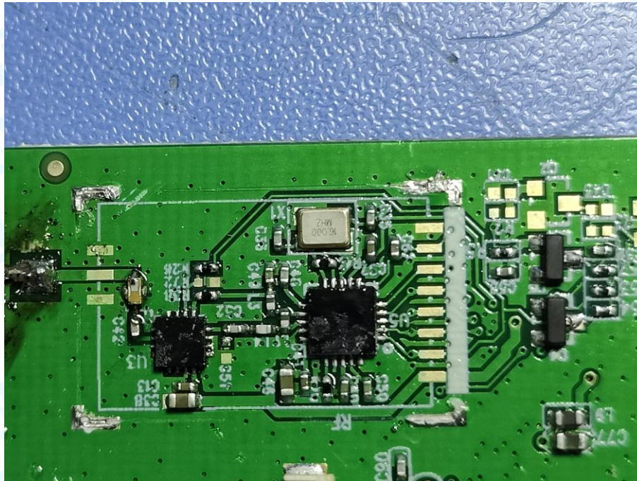
Photo 16 Appearance of PCB (HB6233)
