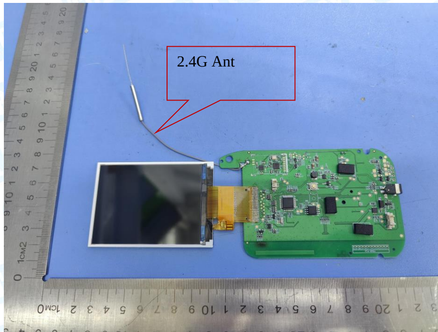
Photo 20 Appearance of PCB Differential prototype 2# (HB6339)
