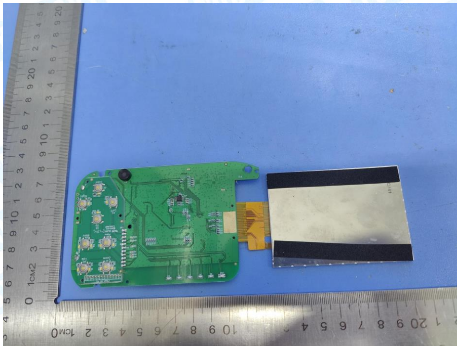
Photo 24 Appearance of PCB Differential prototype 4# (HB6231)
