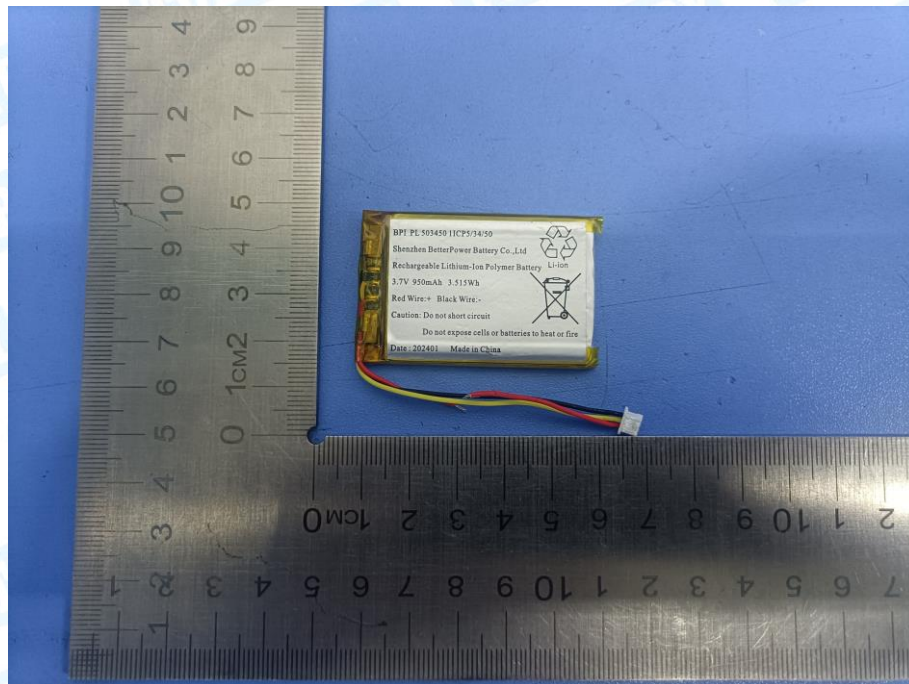
Photo 29 Battery Appearance (BPI PL 503450)
