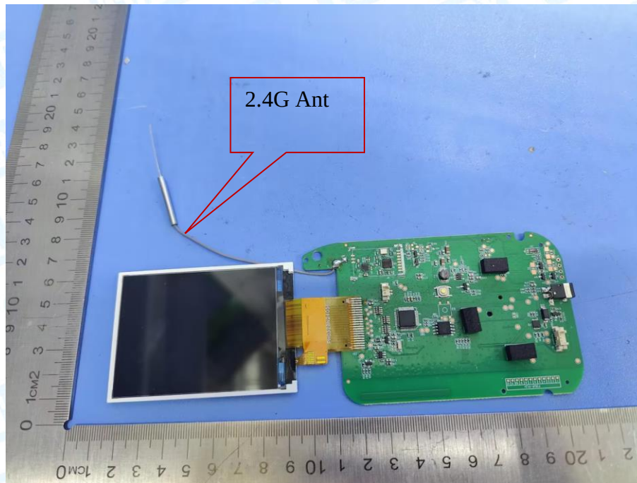
Photo 22 Appearance of PCB Differential prototype 3# (HB2229)
