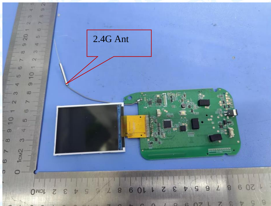
Photo 26 Appearance of PCB Differential prototype 5# (HB2438)
