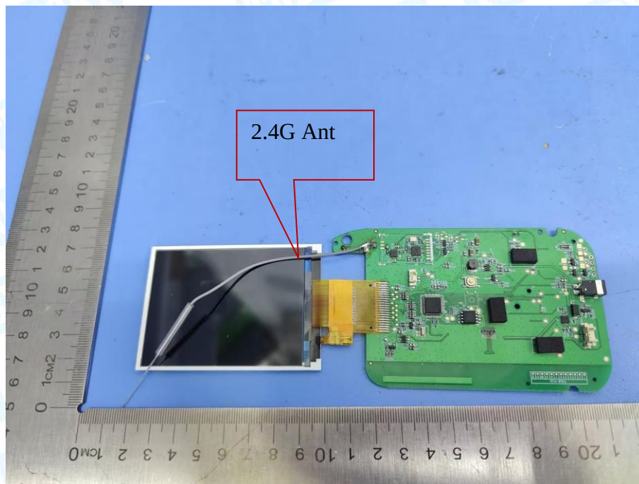
Photo 14 Appearance of PCB (HB6233)
