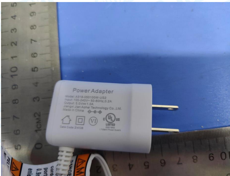
Photo 20 Adapter Appearance 4#
