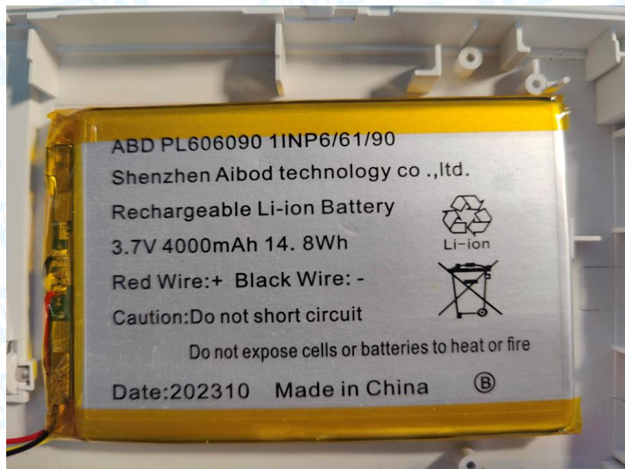
Photo 13 Battery Appearance
