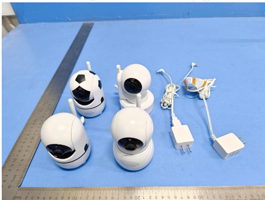
Photo 2 Appearance of EUT(HB60AL_TX)
