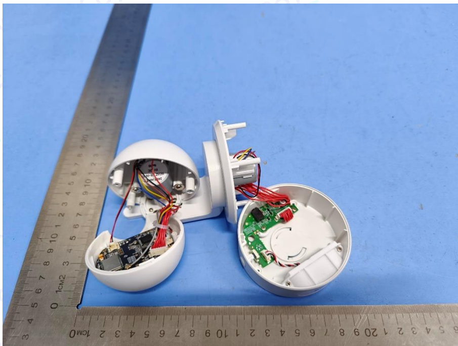
Photo 12 Internal of EUT (HB61AL_TX)
