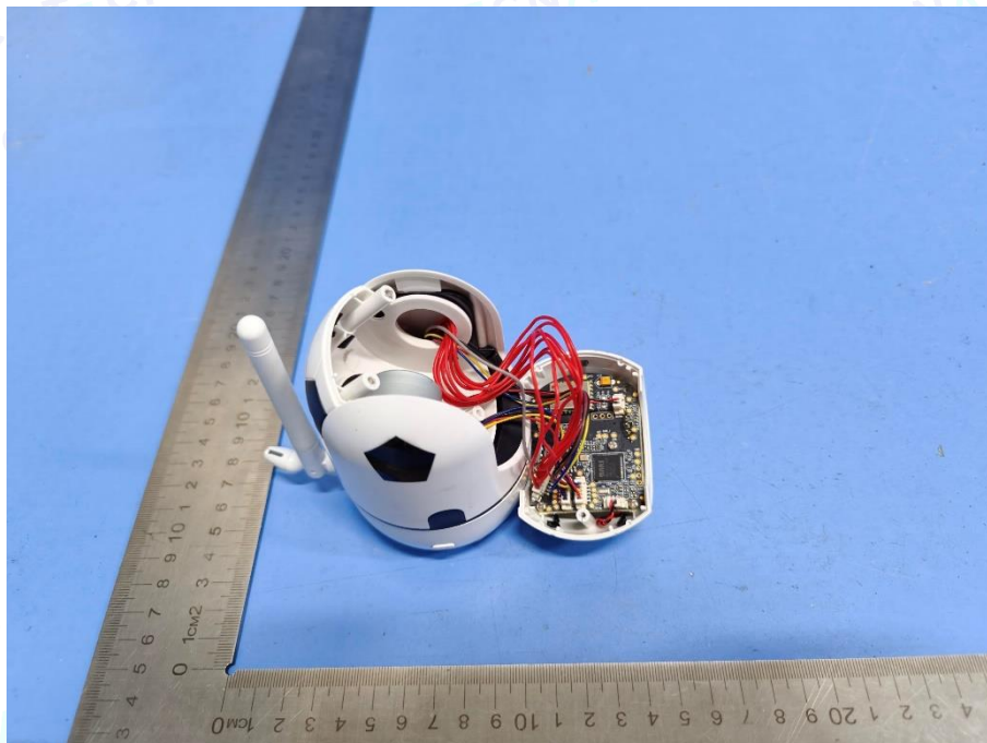
Photo 10 Internal of EUT(HB65AL_TX)
