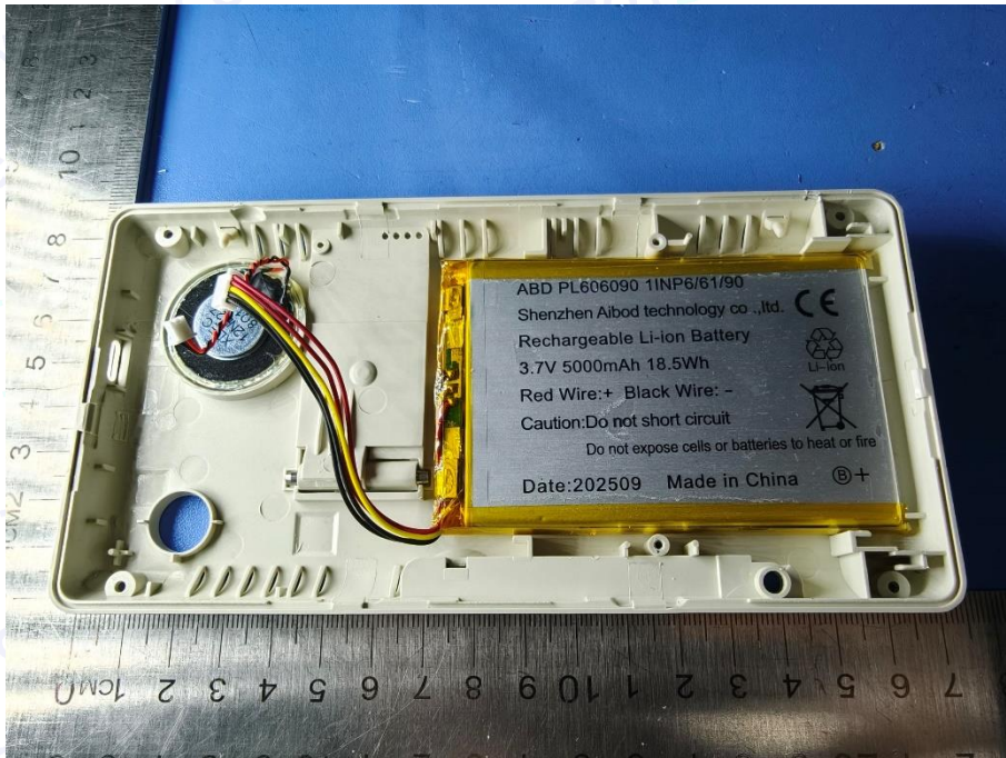
Photo 16 Battery Appearance(11NP6/61/90)
