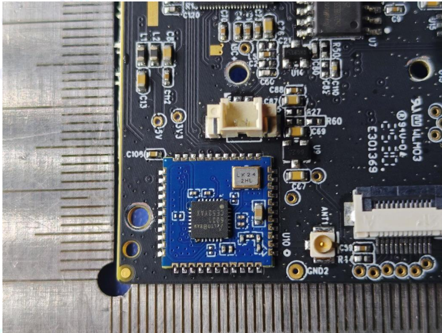
Photo 13 Appearance of PCB (AB6032X-6PE)
