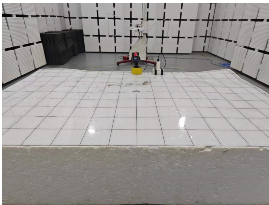
Set-up for Transmitter & Receiver Spurious Emissions, 30MHz to 1000MHz
