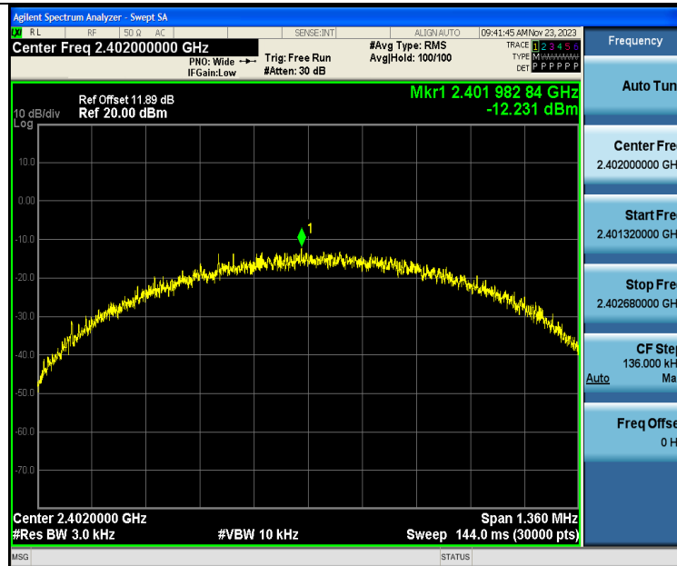
BLE_1M-Ant1-2402-PASS
