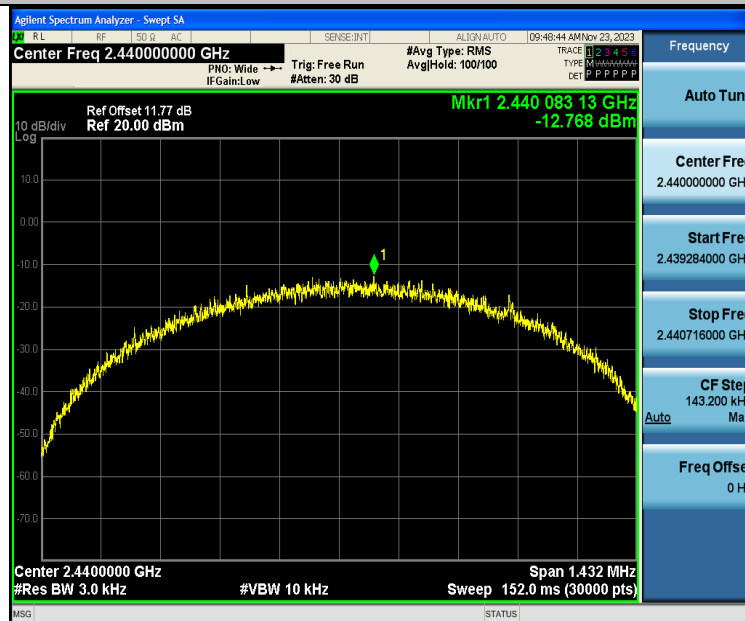
BLE_1M-Ant1-2440-PASS
