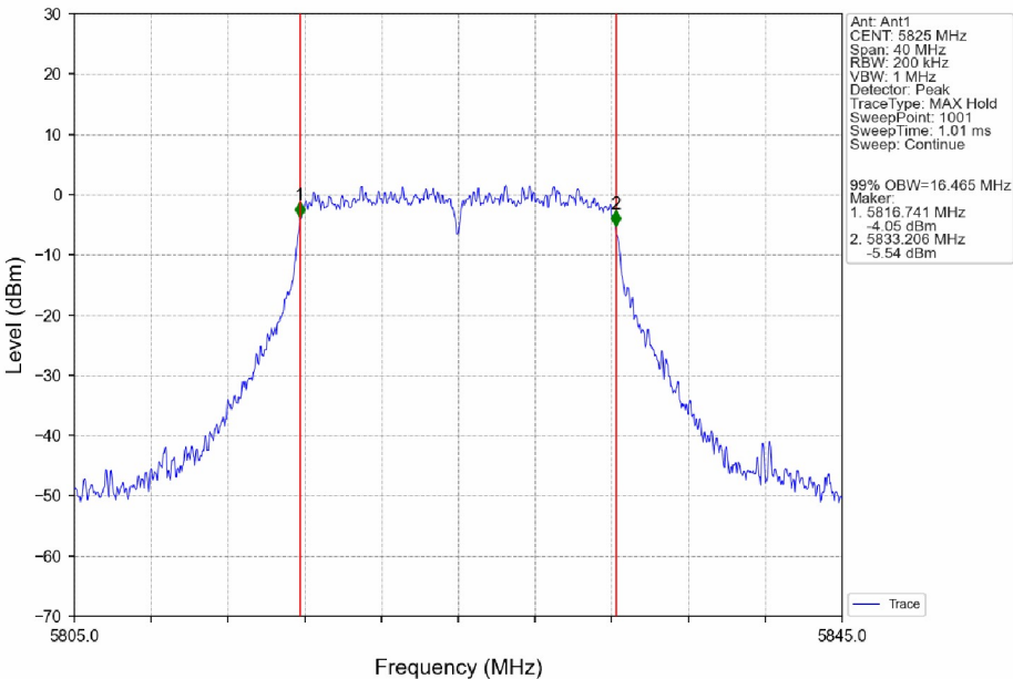
802.11a_HCH_5825MHz_Ant1_NTNV
