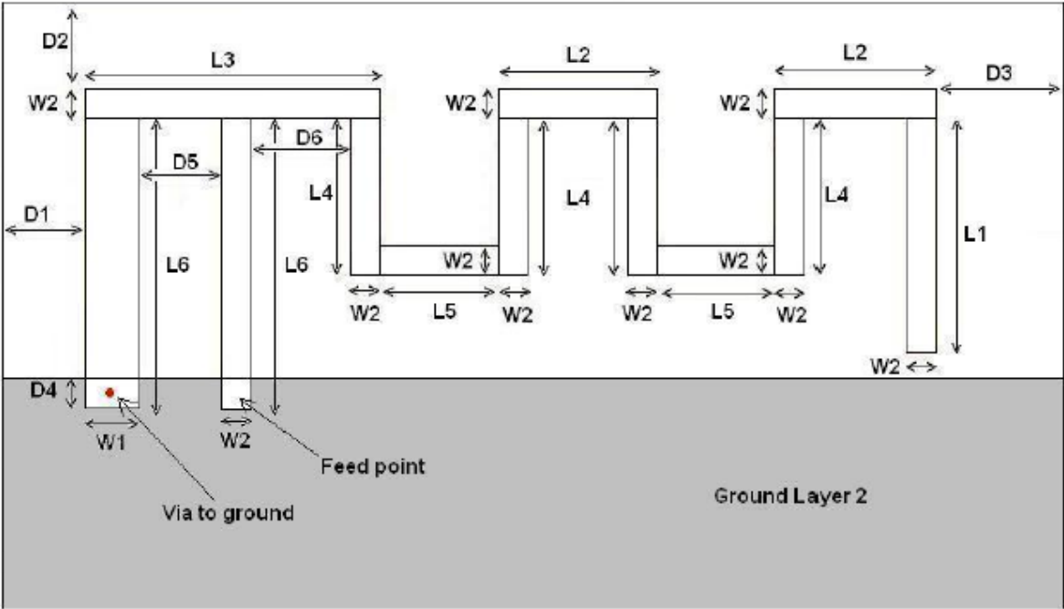
Figure 3: Antenna Dimensions
