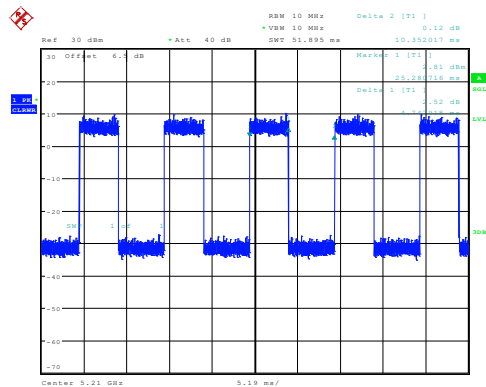
ac80_5210MHz_Chain 0 4.748ms,10.352ms
