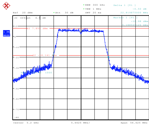
ax20_5200MHz_Chain 0 22.820MHz
