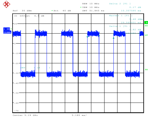
ax40_5190MHz_Chain 0 4.634ms,10.358ms
