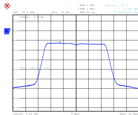
ax20_5240MHz_Chain 0 -2.60dBm/MHz
