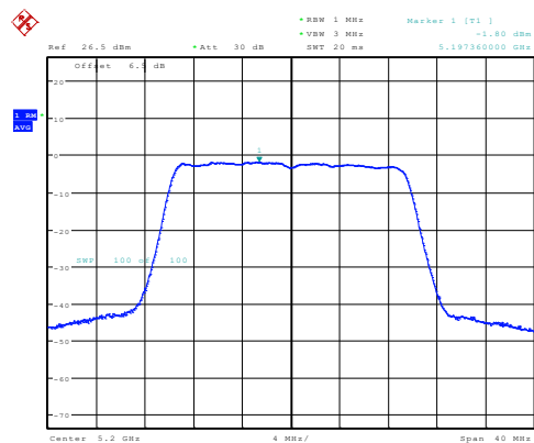
ax20_5200MHz_Chain 0 -1.80dBm/MHz
