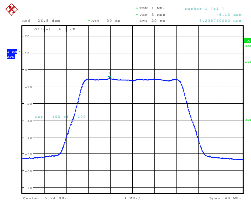
n20_5240MHz_Chain 0 -5.13dBm/MHz
