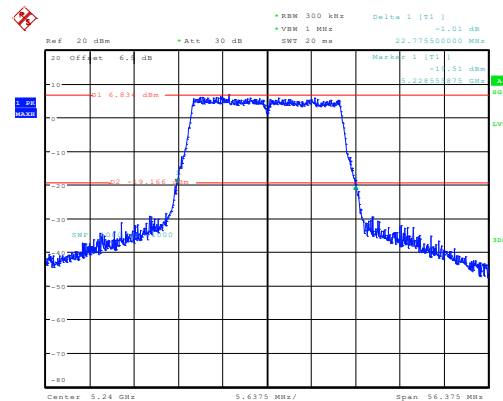
ax20_5240MHz_Chain 0 22.776MHz
