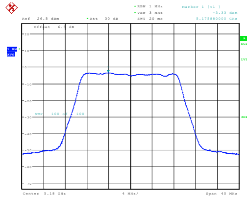
n20_5180MHz_Chain 0 -3.33dBm/MHz
