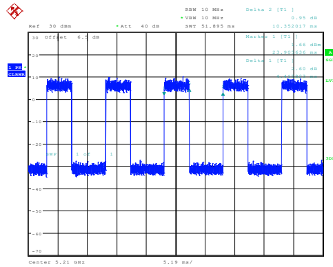
ax80_5210MHz_Chain 0 4.416ms,10.352ms
