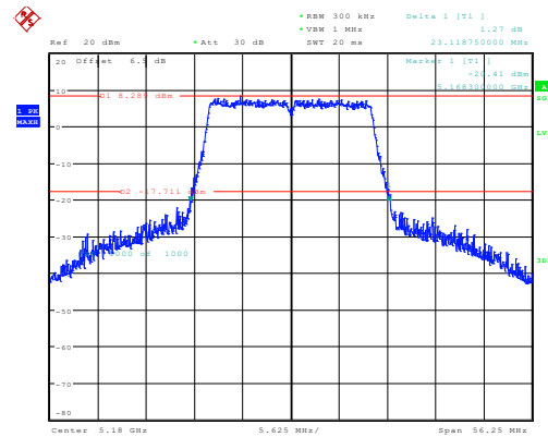
ax20_5180MHz_Chain 0 23.119MHz
