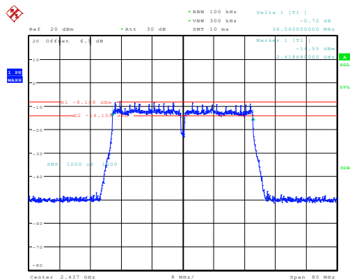
n40_2437MHz_Chain 0 36.560MHz
