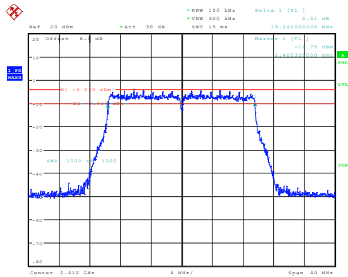
ax20_2412MHz_Chain 0 19.240MHz
