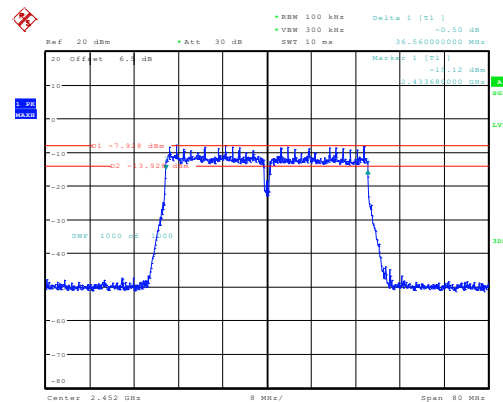
n40_2452MHz_Chain 0 36.560MHz
