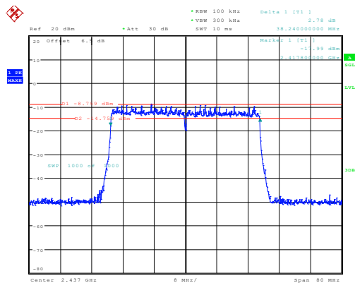
ax40_2437MHz_Chain 0 38.240MHz
