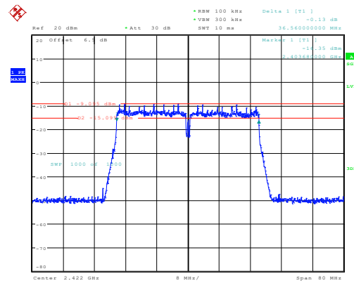
n40_2422MHz_Chain 0 36.560MHz
