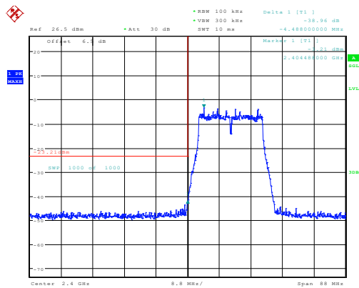
n20_2412MHz_Chain 0 38.96dB
