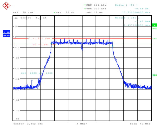
n20_2462MHz_Chain 0 17.720MHz
