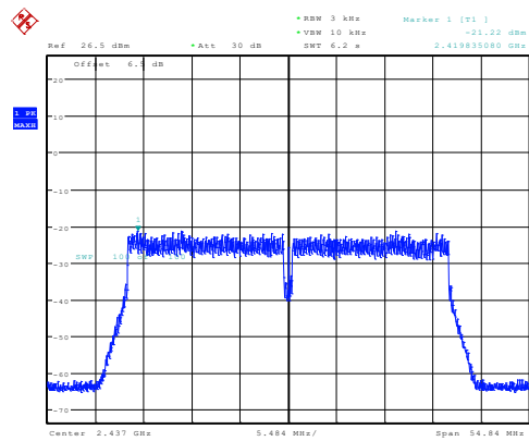
n40_2437MHz_Chain 0 -21.22dBm/3kHz
