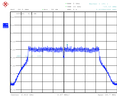
n20_2412MHz_Chain 0 -15.12dBm/3kHz
