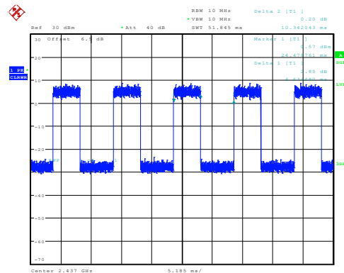
ax40_2437MHz_Chain 0 4.634ms,10.342ms
