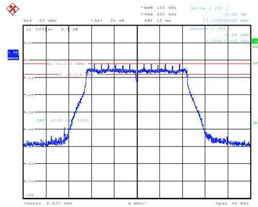
n20_2437MHz_Chain 0 17.720MHz
