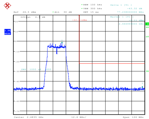
n20_2462MHz_Chain 0 43.32dB
