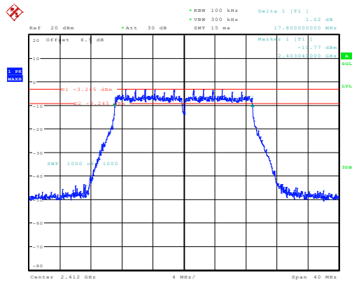
n20_2412MHz_Chain 0 17.800MHz
