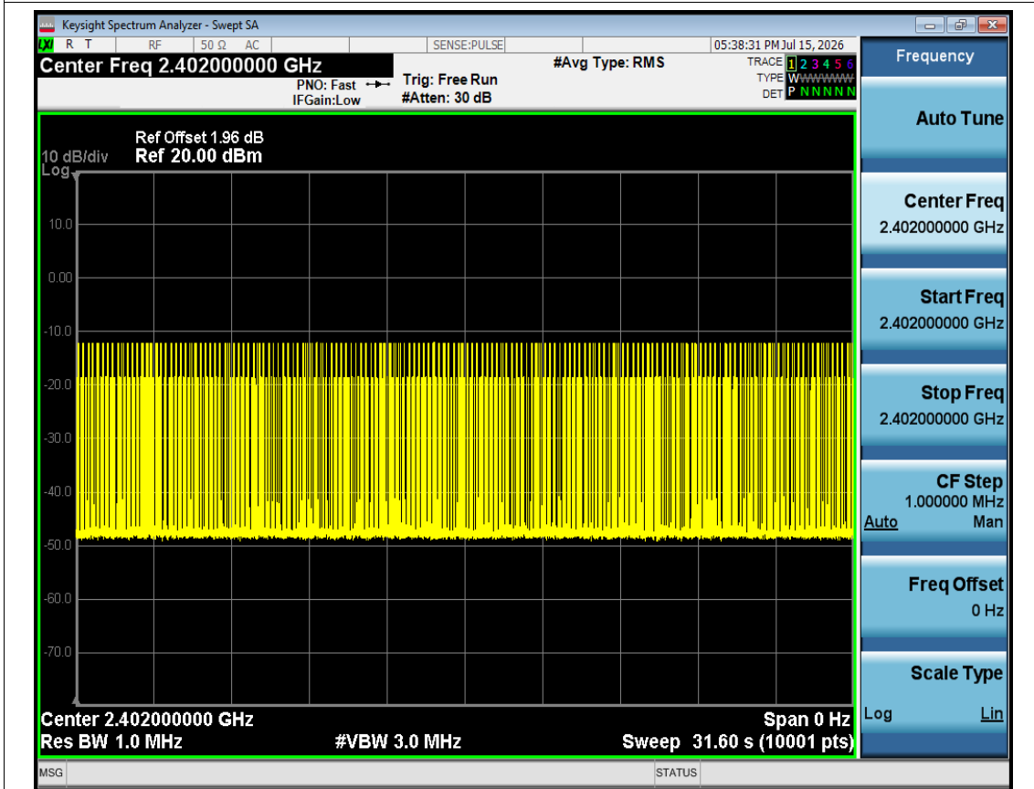
Dwell NVNT 3-DH1 2402MHz Ant1 Accumulated
