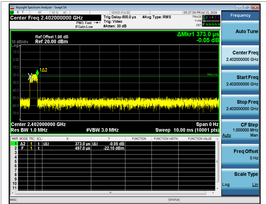
Dwell NVNT 3-DH1 2402MHz Ant1 One Burst
