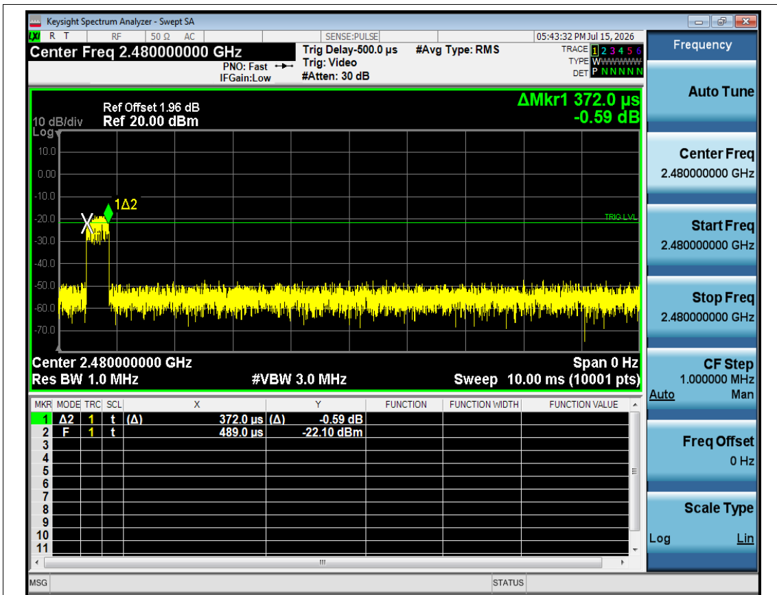
Dwell NVNT 3-DH1 2480MHz Ant1 One Burst
