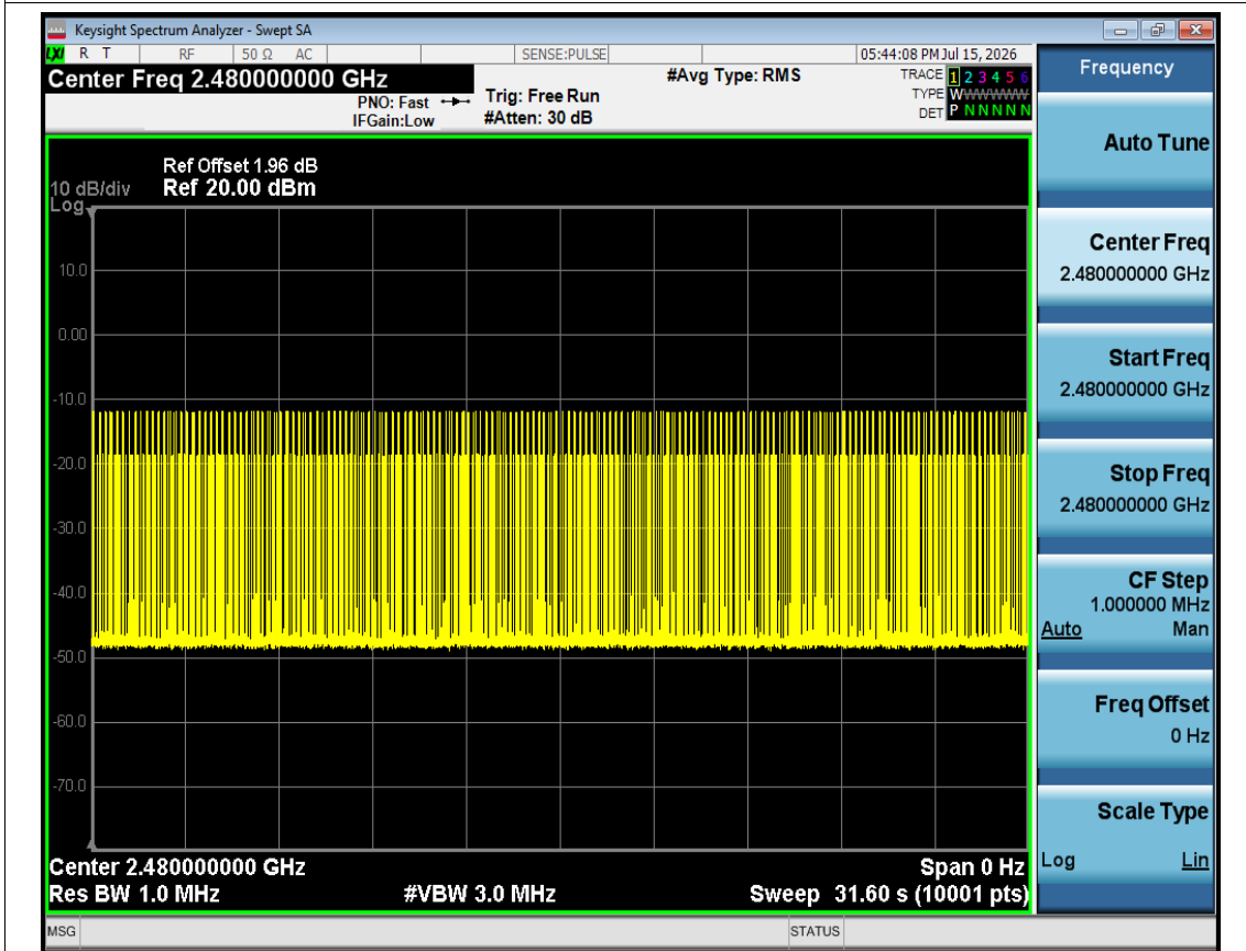
Dwell NVNT 3-DH1 2480MHz Ant1 Accumulated
