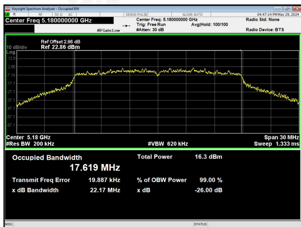
(802.11ac20) 99%Bandwidth plot on channel 36
