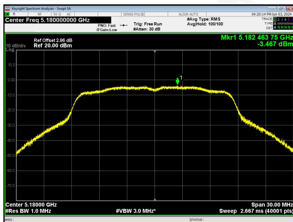
ANT2 (802.11a) PSD plot on channel 36
