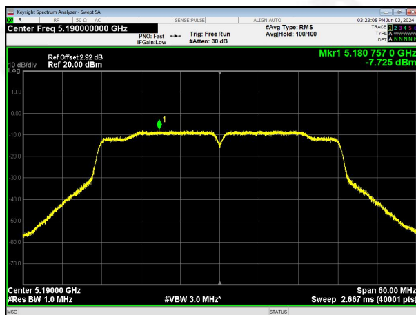
ANT1 (802.11ac40) PSD plot on channel 38
