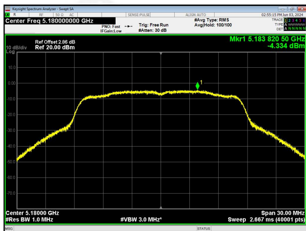
ANT1 (802.11a) PSD plot on channel 36
