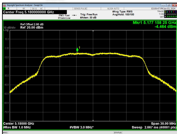
ANT1 (802.11ac20) PSD plot on channel 36
