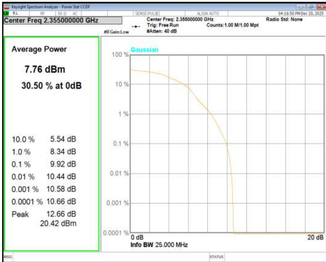
Band40(2350-2360) 16QAM BW=5MHz Channel=39175 RB Size=1 Position=#0
